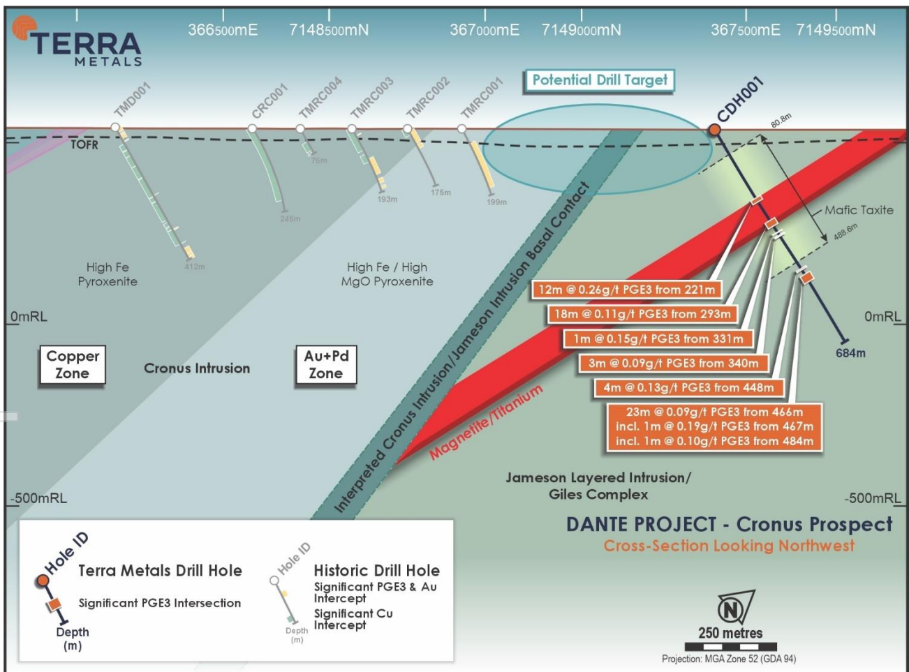
Figure 9. Cronus geological cross section
