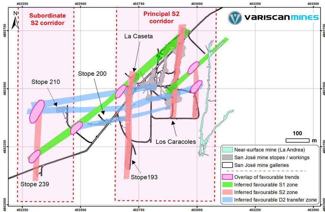
Figure 6. Plan view of structural trends at the San Jose Mine 2
