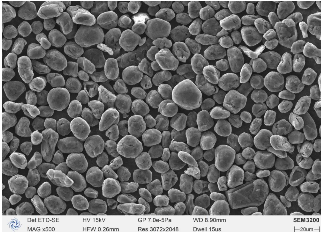
Figure 1: Scanning Electron Microscope image of CSPG produced from Upgraded Malingunde Concentrate showing conventional potato-shaped particles
