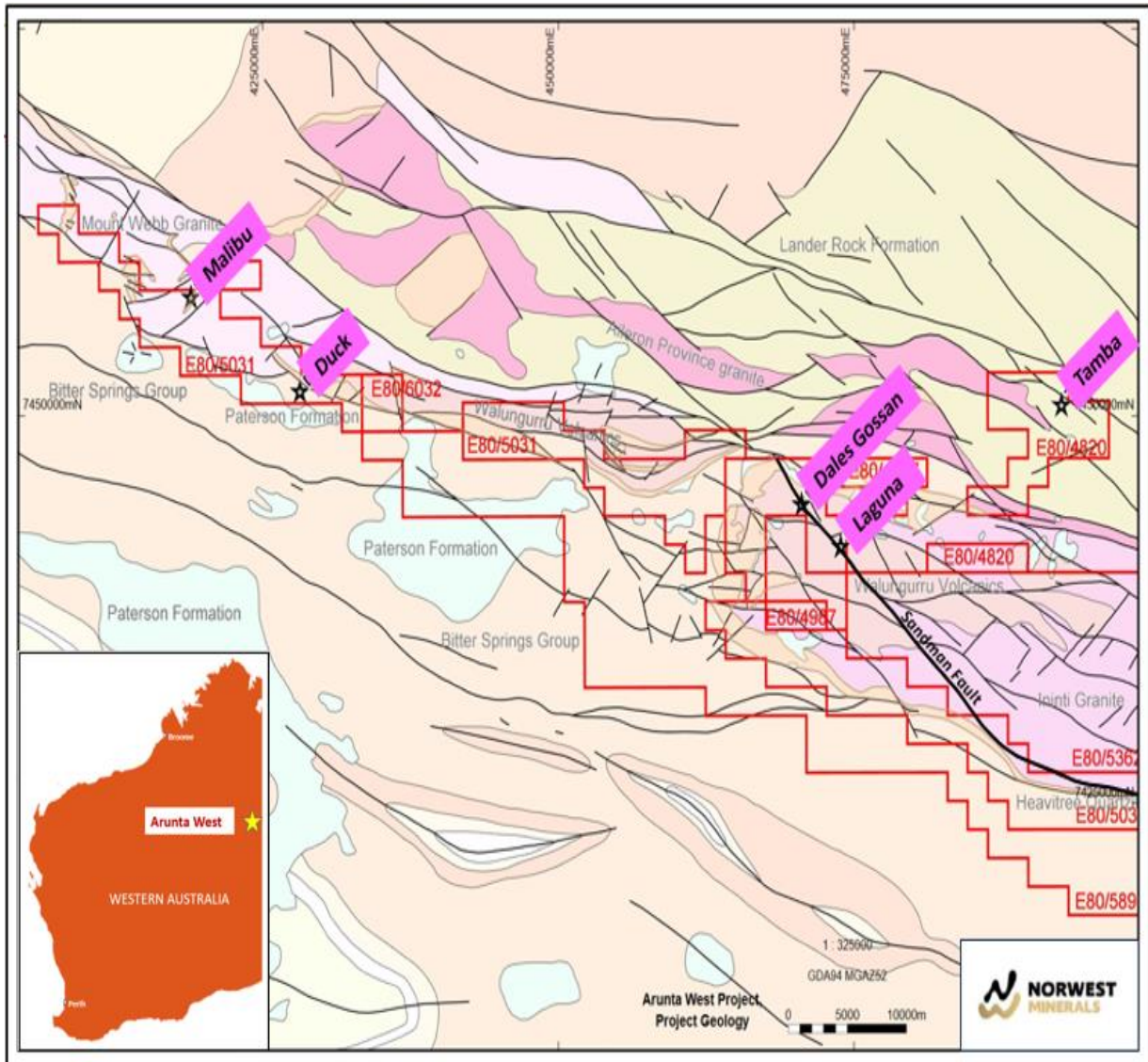
Figure 2 – Arunta West tenement and prospect location map with Sandman fault.
