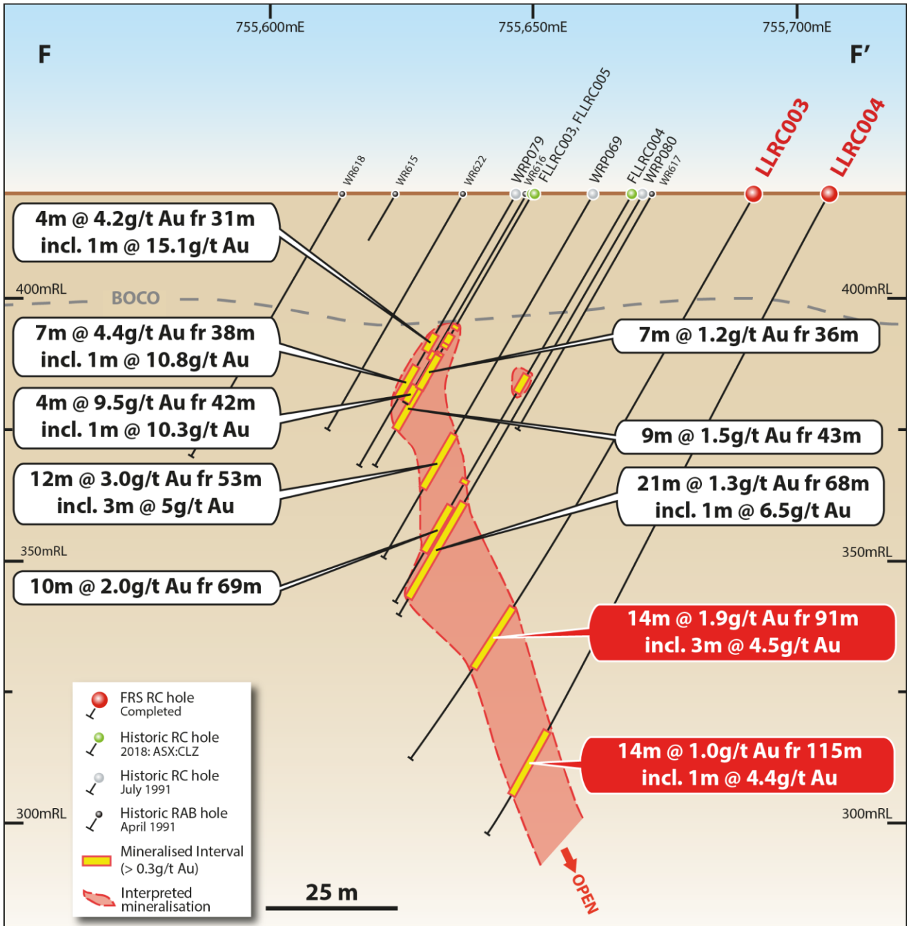
Figure 4. Cross section (F-F'), looking north ~15m along strike, showing Au mineralisation of historic and FRS drilling. Drilling intercept widths are down-hole widths and not true widths. Intercepts are based on a cut-off grade of 0.3g/t Au, allowing for internal dilution by two "waste" or sub-grade (<0.3g/t Au) samples. FRS holes (red caption) were completed in 2021.
