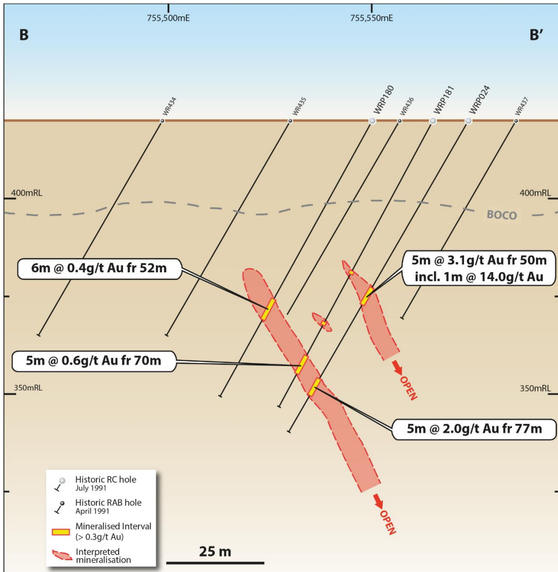
Figure 9. Cross section (B-B'), looking north ~10m along strike, showing Au mineralisation of historic drilling. Drilling intercept widths are down-hole widths and not true widths. Intercepts are based on a cut-off grade of 0.3g/t Au, allowing for internal dilution by two "waste" or sub-grade (<0.3g/t Au) samples.
