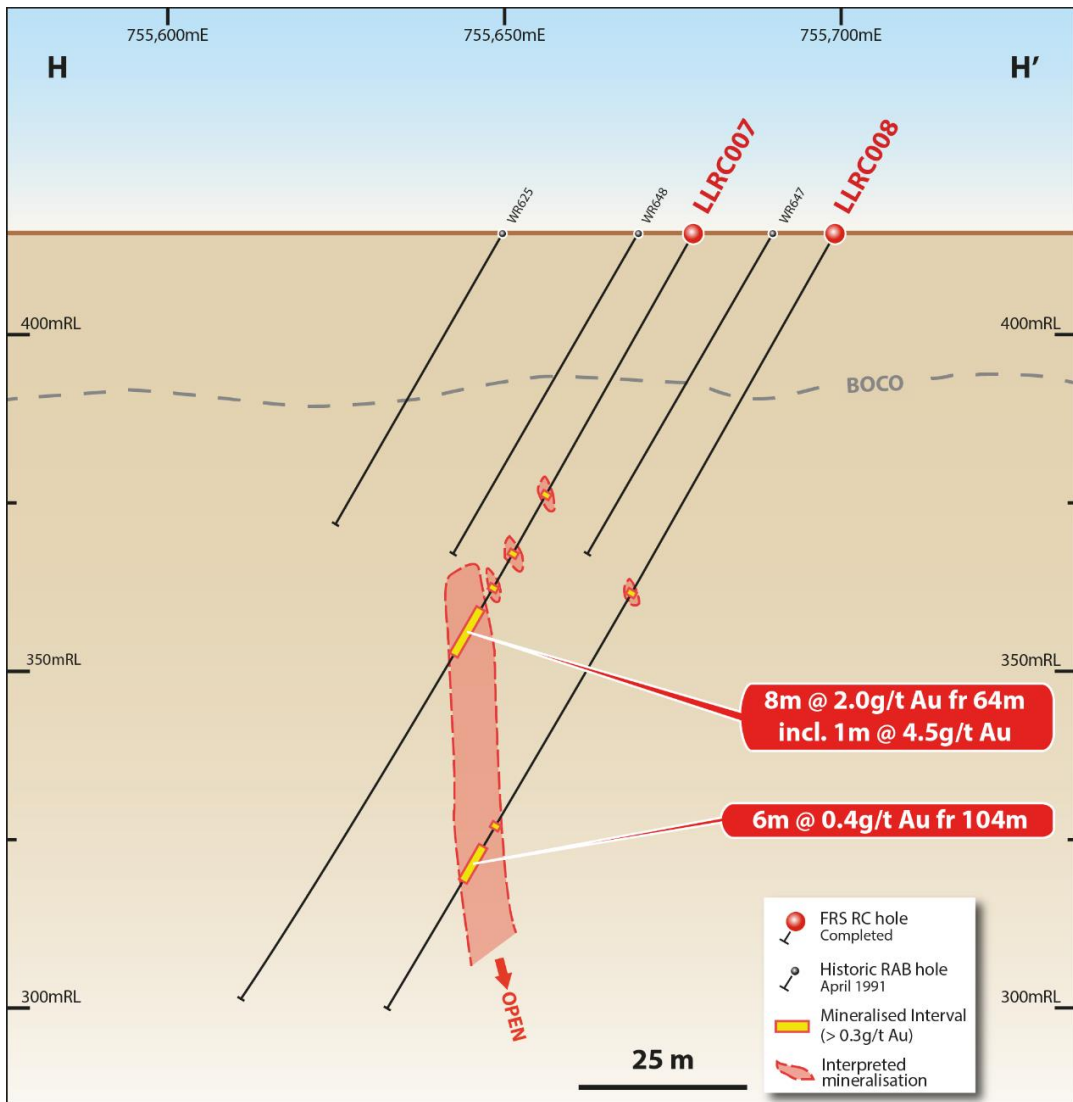
Figure 11. Cross section (H-H'), looking north ~10m along strike, showing Au mineralisation of historic & FRS drilling. Drilling intercept widths are down-hole widths and not true widths. Intercepts are based on a cut-off grade of 0.3g/t Au, allowing for internal dilution by two “waste” or sub-grade (<0.3g/t Au) samples. FRS holes (red caption) completed in 2021.
