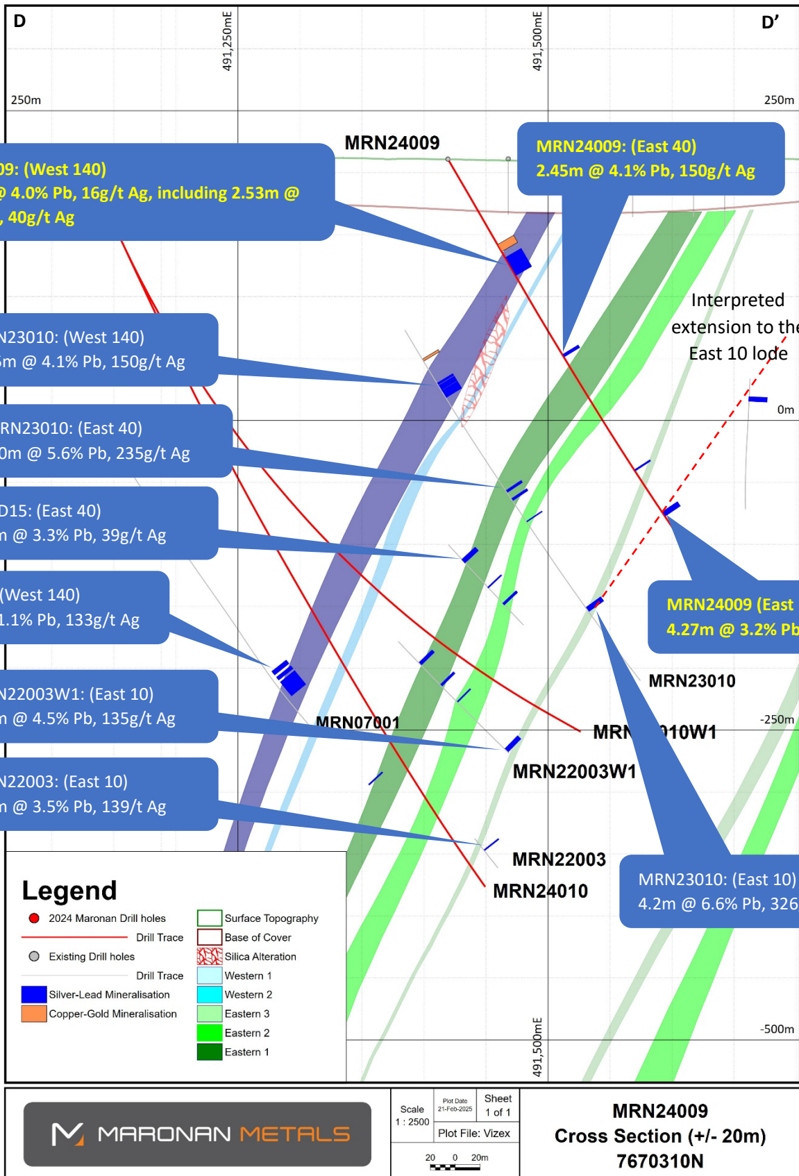
Figure 10: Working cross section looking north showing MRN24009 highlighting the context of intercepts on the Western and Eastern Horizons. MRN24009 has led to a re-interpretation of the East 10 lode in conjunction with MRN24008.
