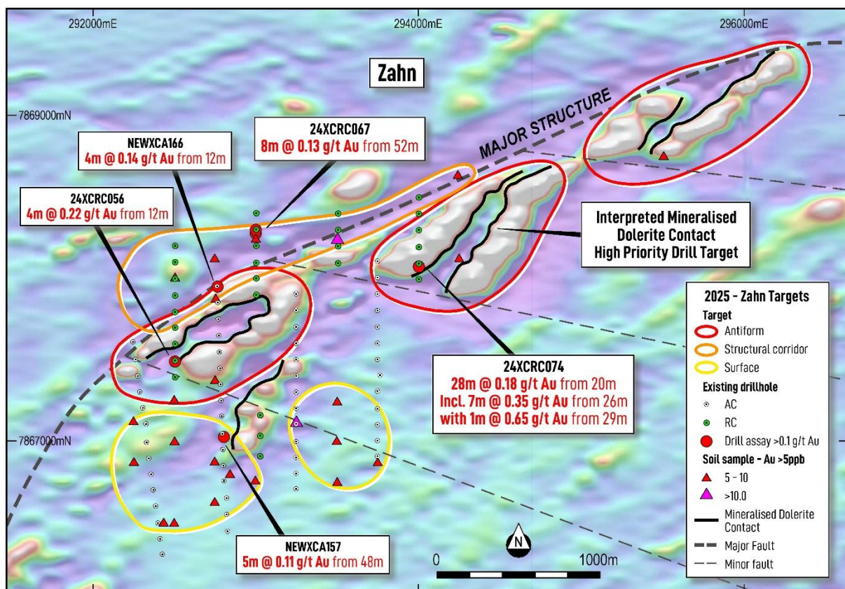
Figure 1. Plan view of the Zahn Prospect area, showing target zones, drilling with significant intercept callouts and selected soil samples above 5ppb Au. The background image is magnetics (TMI RTP 1VD) and shows an interpreted early high-mag intrusive that has been folded, providing antiformal structures adjacent to a demagnetised structural corridor / Major Structure. The interpreted antiformal dolerite contacts represent high priority drill targets for the upcoming field program.
