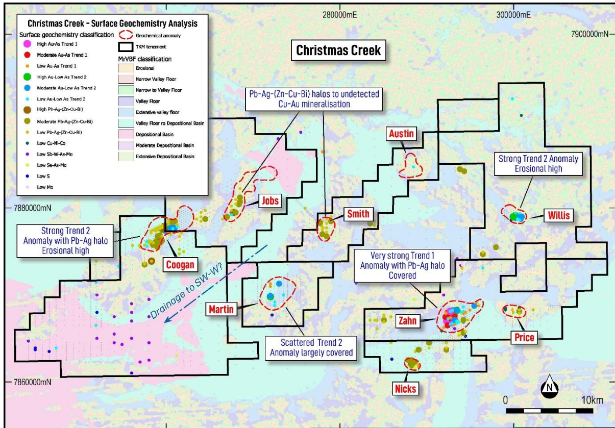
Figure 2. Categorized surface geochemical responses at the greater Christmas Creek Project area highlight the large multi-square-kilometre responses associated with the Coogan and Zahn Prospect areas.
