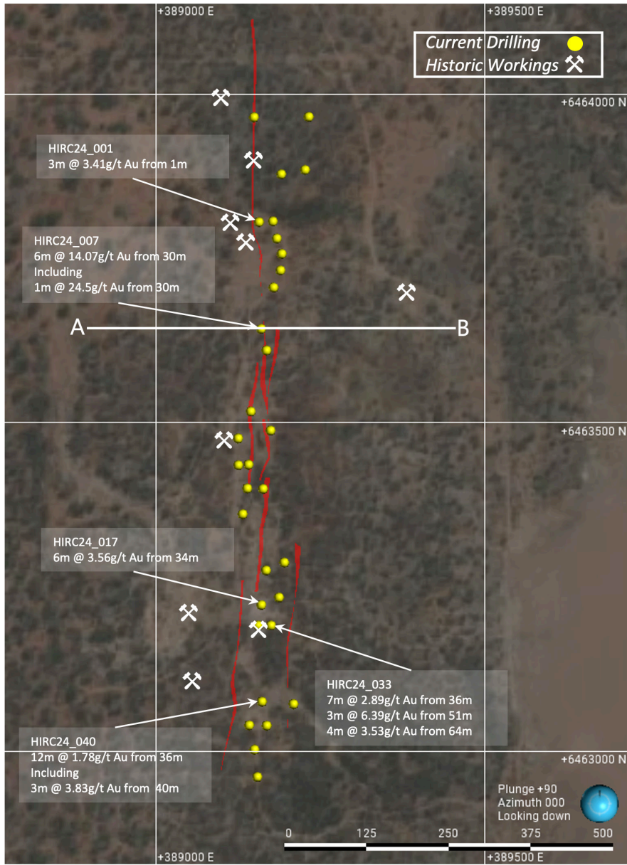
Figure – Plan view of drilling.
