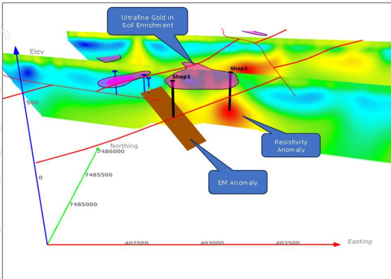
Figure 4. 3D image looking northeast showing surface geochemistry and key geophysical features and structural trends, (Brown is FLEM plate model, coloured sections are resistive IP, and red lines are interpreted structural trends)
