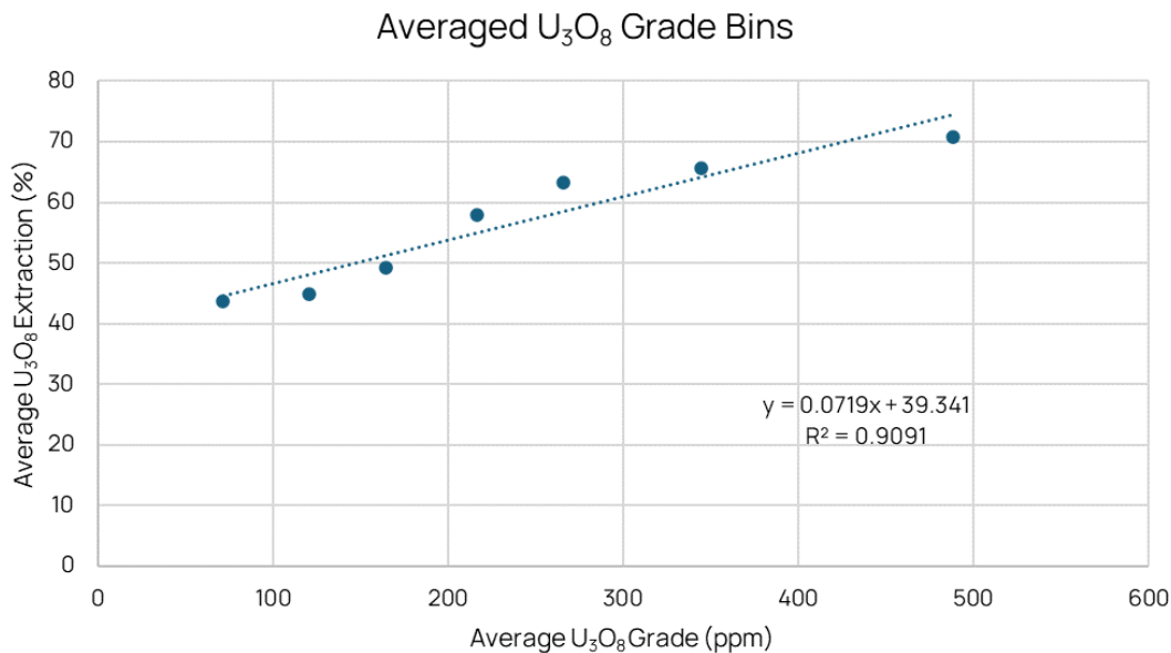
Figure 6: Lethakane uranium extraction vs mill feed grade
