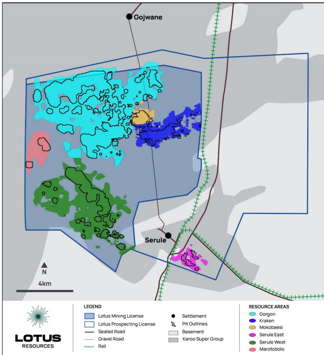
Figure 2: Lethlakane deposit and pit shells
