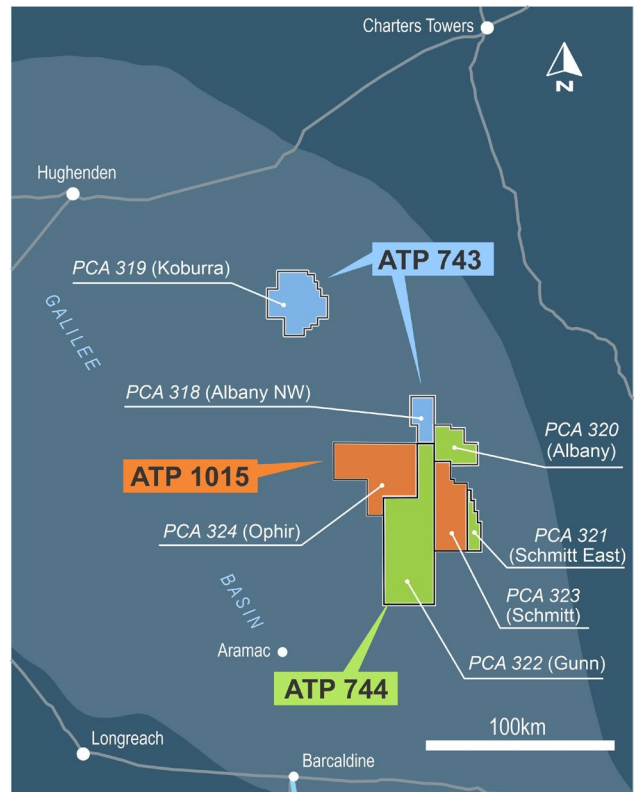
Figure 3 – Galilee permits showing the recently awarded PCAs within permits ATP 743, ATP 744 and ATP 1015
