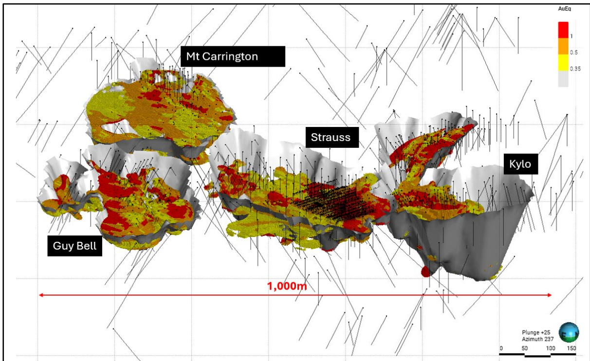
Figure 2: Oblique 3D view looking SW - drillholes and resource AuEq block models (>0.35g/t AuEq) across the Mt Carrington Group (>0.5g/t AuEq – Orange, >1g/t AuEq – Red) and RPEEE pit shells. The resource remains open with geophysical IP chargeability targets, indicating mineralisation continues along strike and down dip.
