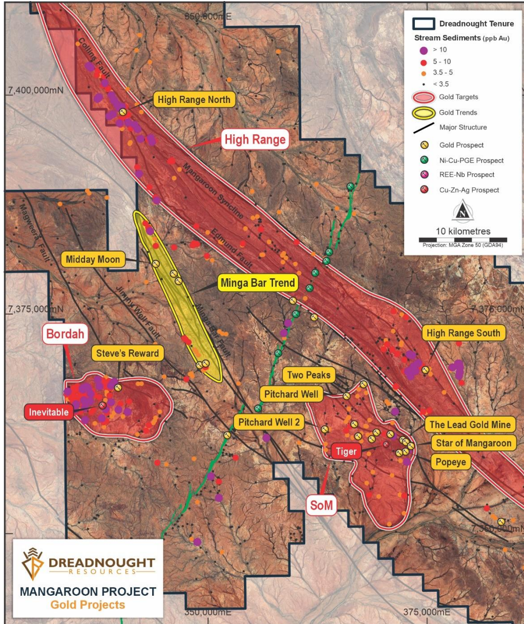
Figure 4: Plan view image of a portion of Mangaroon highlighting the main gold camp scale prospects and targets.
