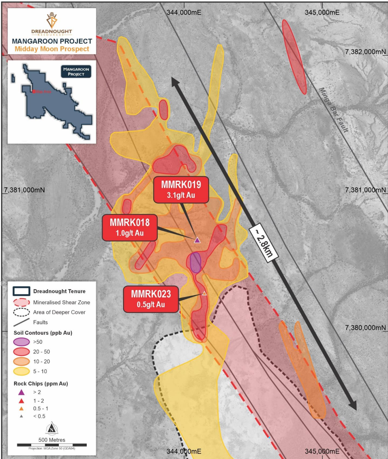
Figure 3: Plan view image of Midday Moon showing the gold in soil anomaly contours over 2.8 kms and the location of confirmed gold mineralisation and major structures.
