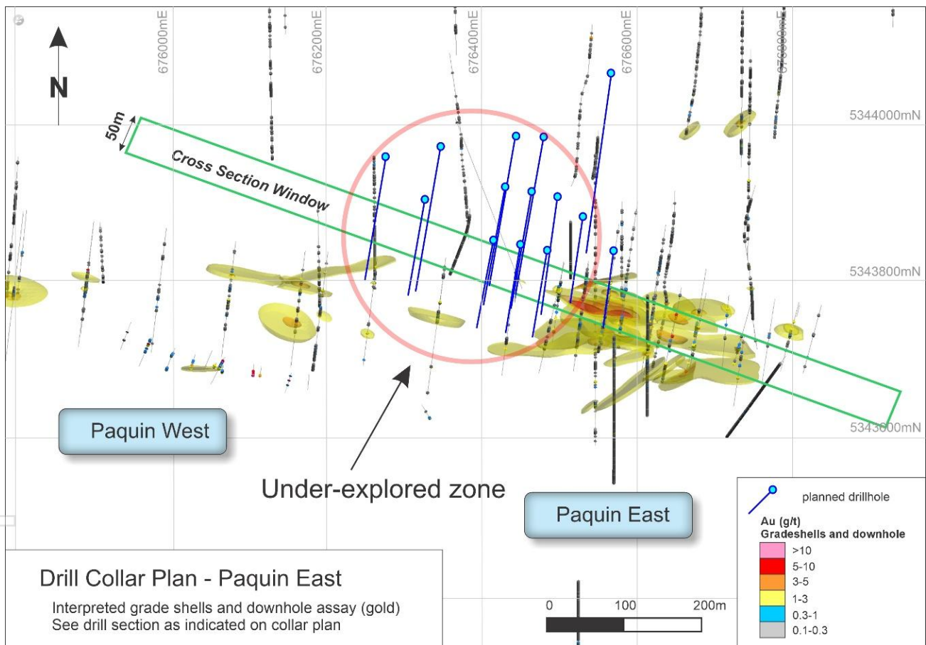
Figure 3: Paquin East drill collar plan with interpreted grade shells and downhole assays. See cross section Fig. 2.
