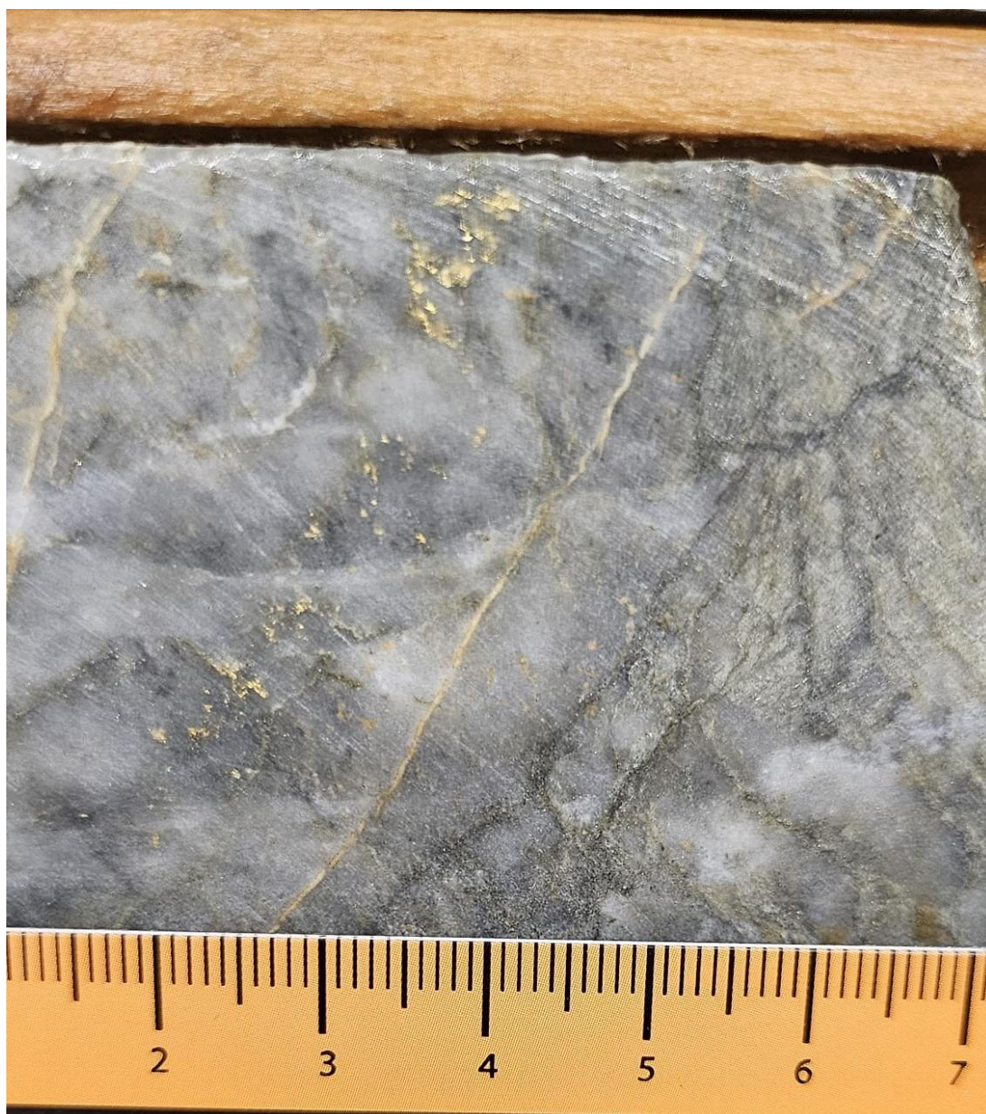
Figure 4: Photo of core from drillhole B0-21-08 at the Paquin East prospect showing visible gold within characteristic blue-grey quartz (184.5m). Scale unit is centimetres. The one metre interval 184-185m assayed 1m@ 129.25g/t Au, within 9m @ 16.96g/t Au from 178.5m 6
