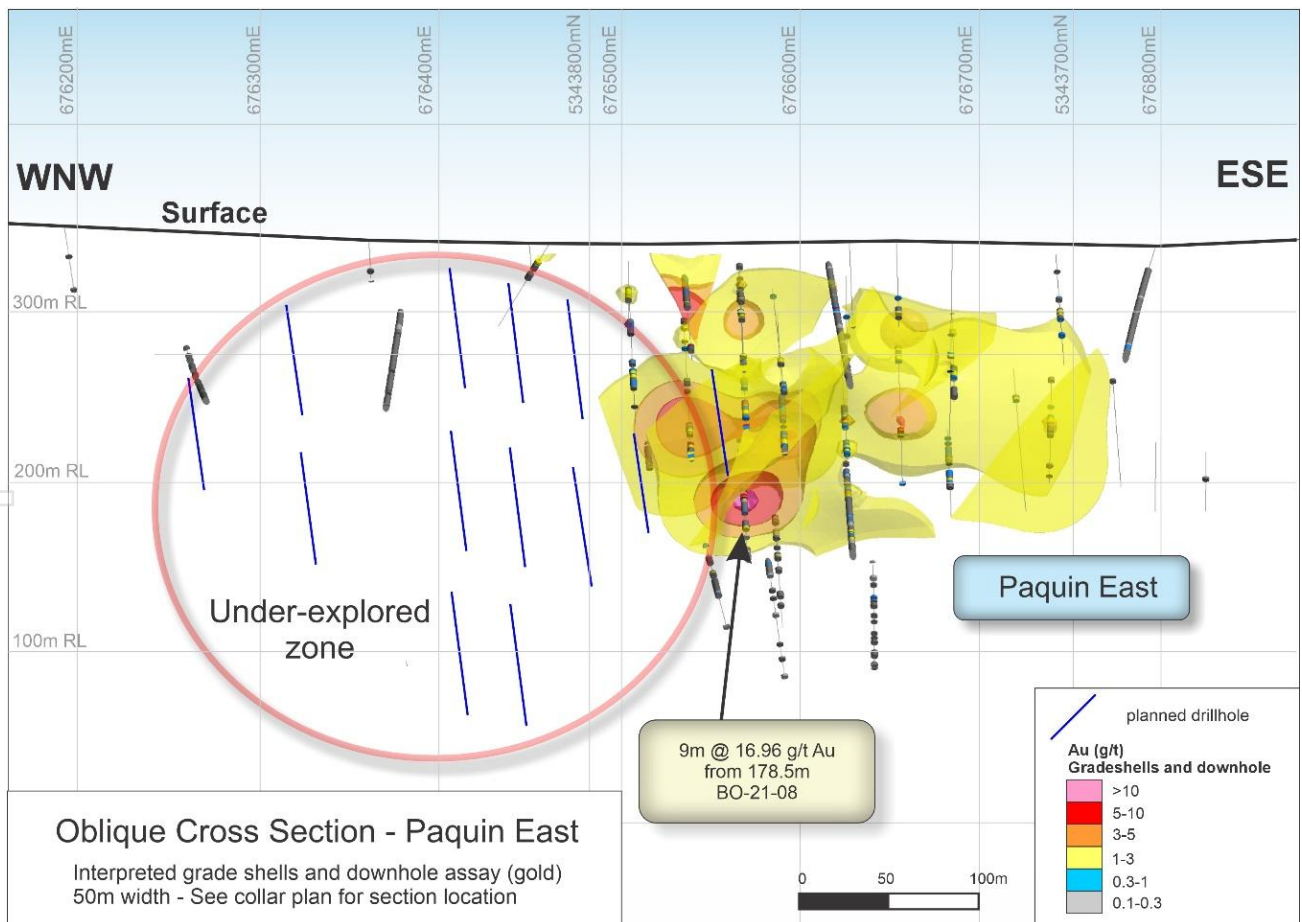
Figure 2: Paquin East oblique cross section with interpreted grade shells and downhole assays. See collar plan Fig. 3.
