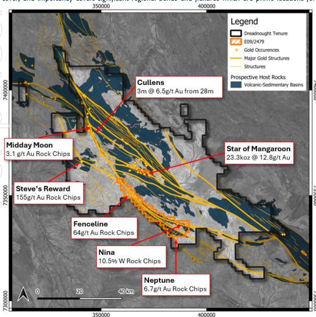
Figure 1: Plan view image showing the location of E092479 in relation to the wider Mangaroon Project and gold occurrences.
