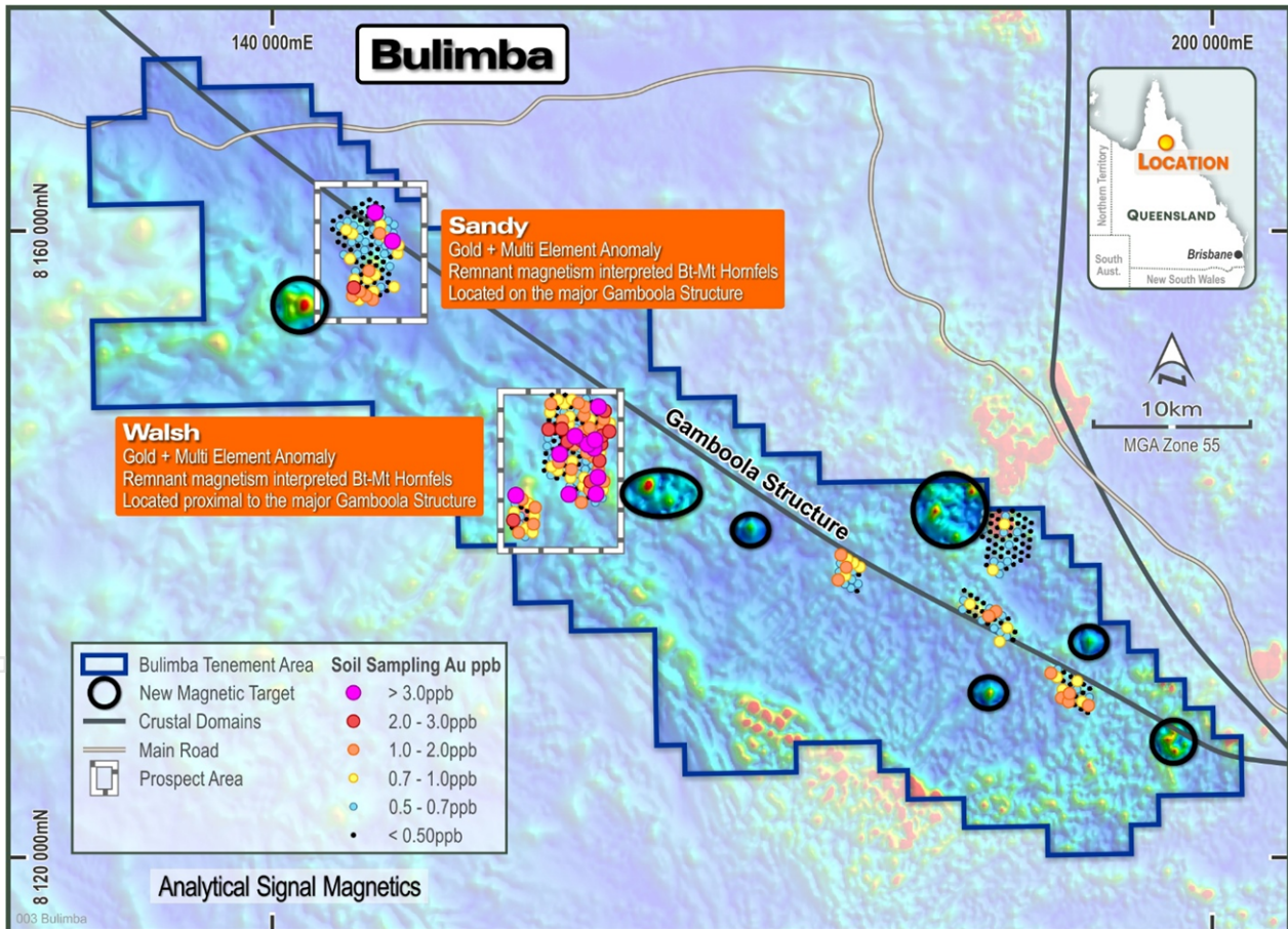
Figure 4: The Sandy and Walsh Prospects with gold geochemistry over Analytical Signal magnetic image.
