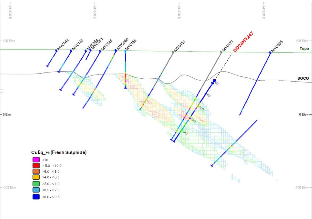
Figure 4: Cross section through Trilogy block model (CuEq %), section line shown in Annexure 3.
