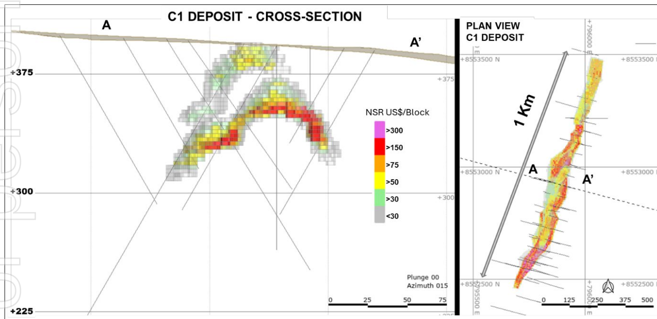
Figure 7: C1 deposit with 3D block model in central cross-section with NSR, drilling and Plan View (RHS).
