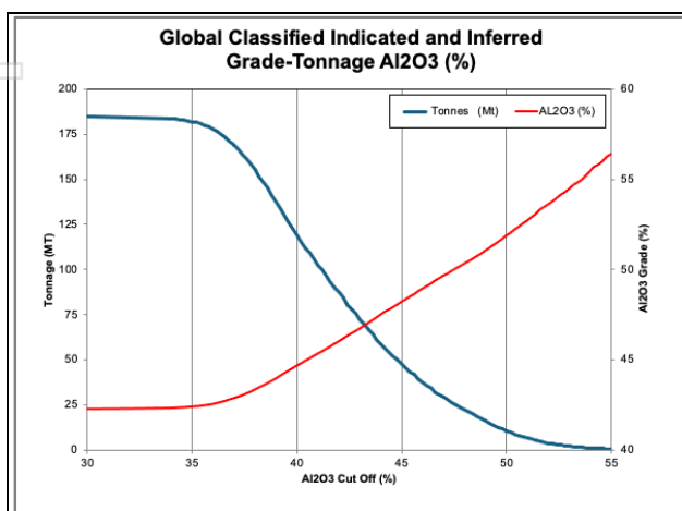
Figure 3. Grade-Tonnage for Global Indicated and Inferred Mineral Resource - Al 2 O 3 (%)
