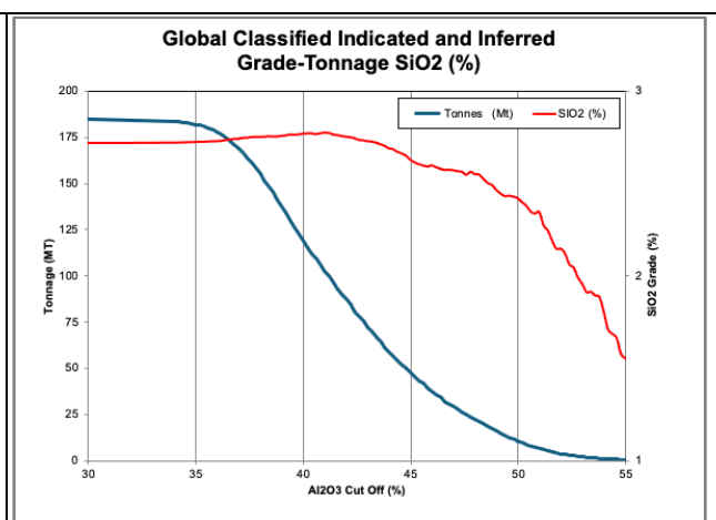
Figure 4. Grade-Tonnage for Global Indicated and Inferred Mineral Resource - SiO 2 (%)
