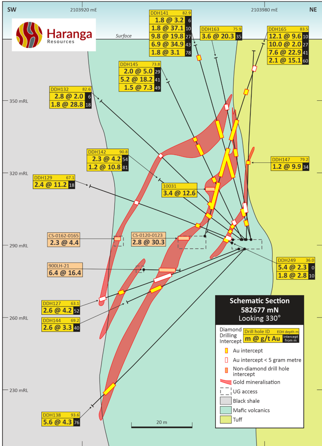
Figure 5: Section line from figure 4 showing Veins hosted within mafic unit, as defined from drilling (Drillhole Table Appendix 1).
