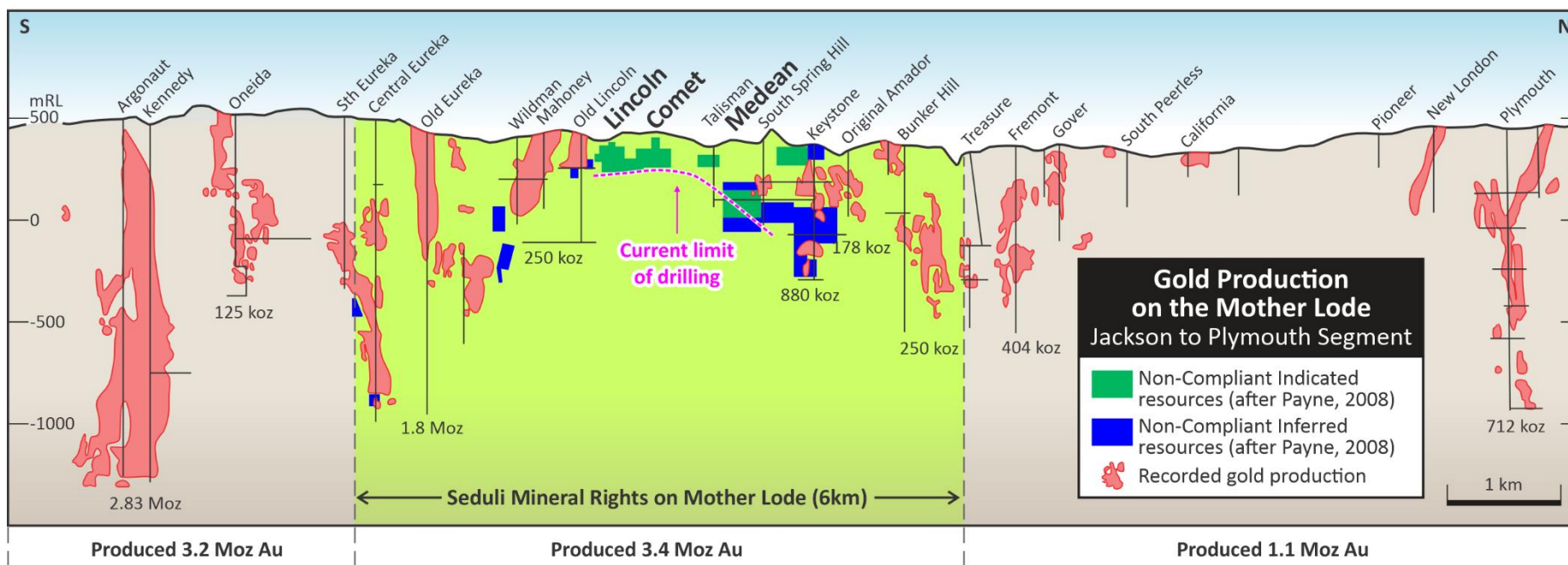
Figure 9: Plan and Long Section of Resources ( Non-JORC Compliant ) taken from Payne 5 (2008, pp61) illustrating the scope of mineralisation identified from historic sampling at Keystone (South Spring Hill).
