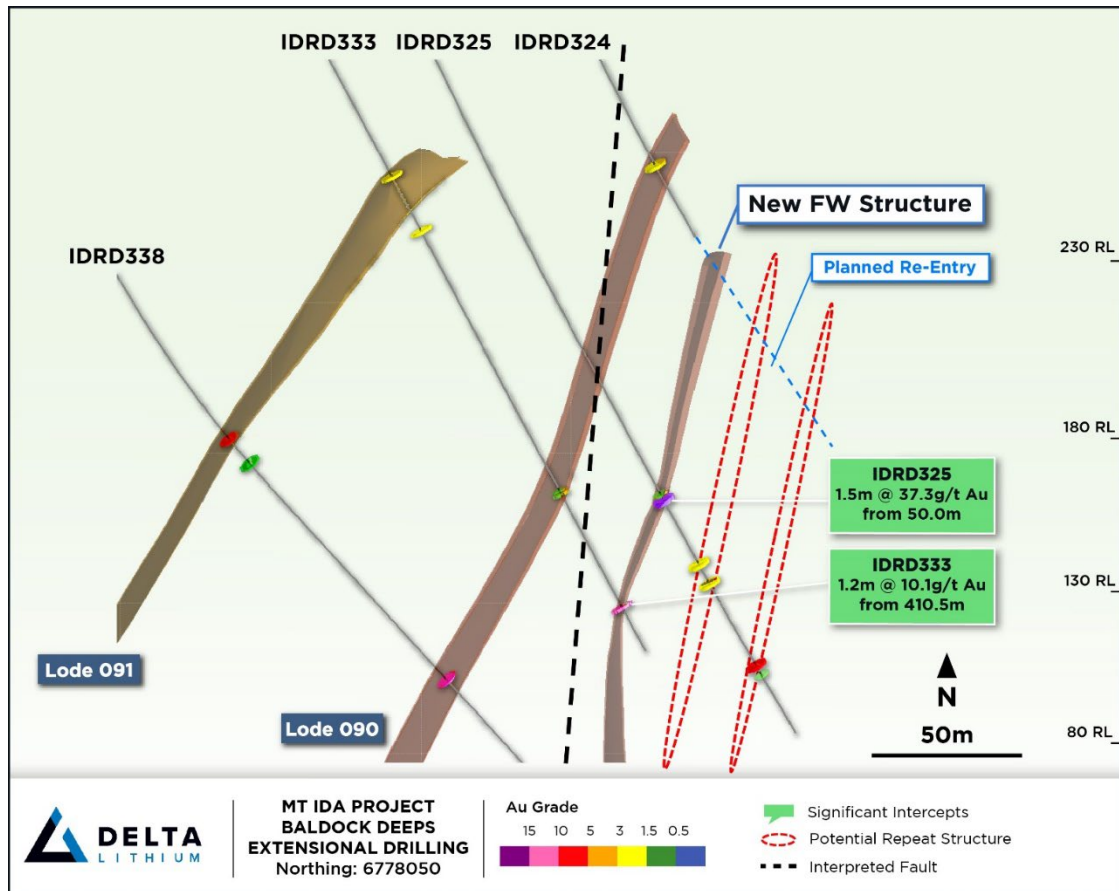
Figure 2: Cross-section showing Baldock deep lodes beyond the current MRE and new high-grade structure that remains open to the South. (Refer to white dashed line in Figure 3 for location of cross section)
