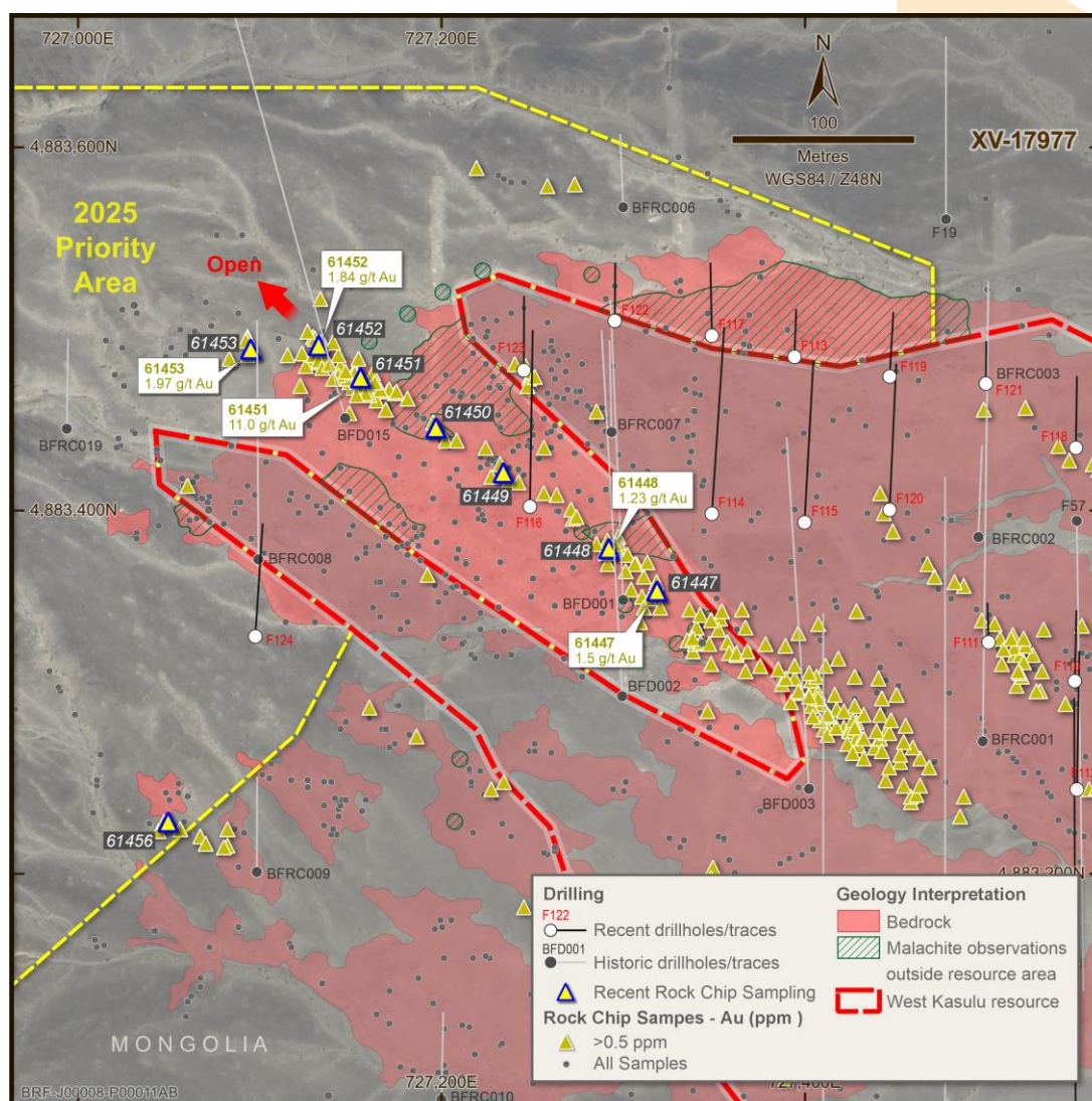
Figure 3: Bronze Fox Project – West Kasulu prospect showing high-grade gold trend towards the northwest.
