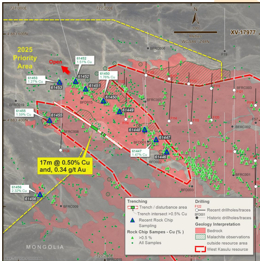
Figure 2: Bronze Fox Project – West Kasulu prospect showing high-grade copper trend towards the northwest.
