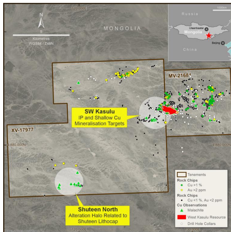
Figure 1: Bronze Fox Project showing priority targets
