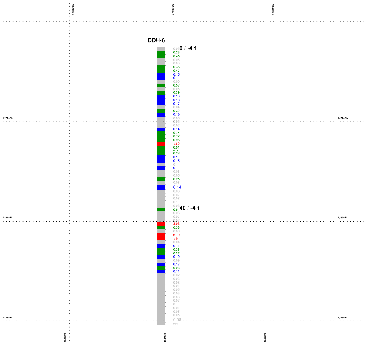
Figure 5: Cross Section of drillhole DDH-6 (drilled to ~70m depth) that shows typical downhole distribution of gold mineralisation in oxide rocks. Note that copper was not analysed for in drillholes.
