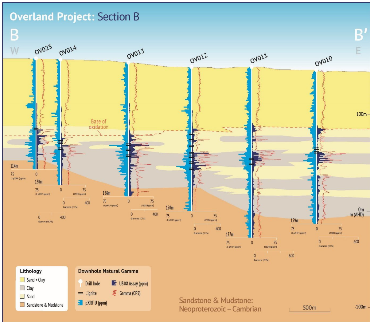
Figure 5: Section B-B 1
