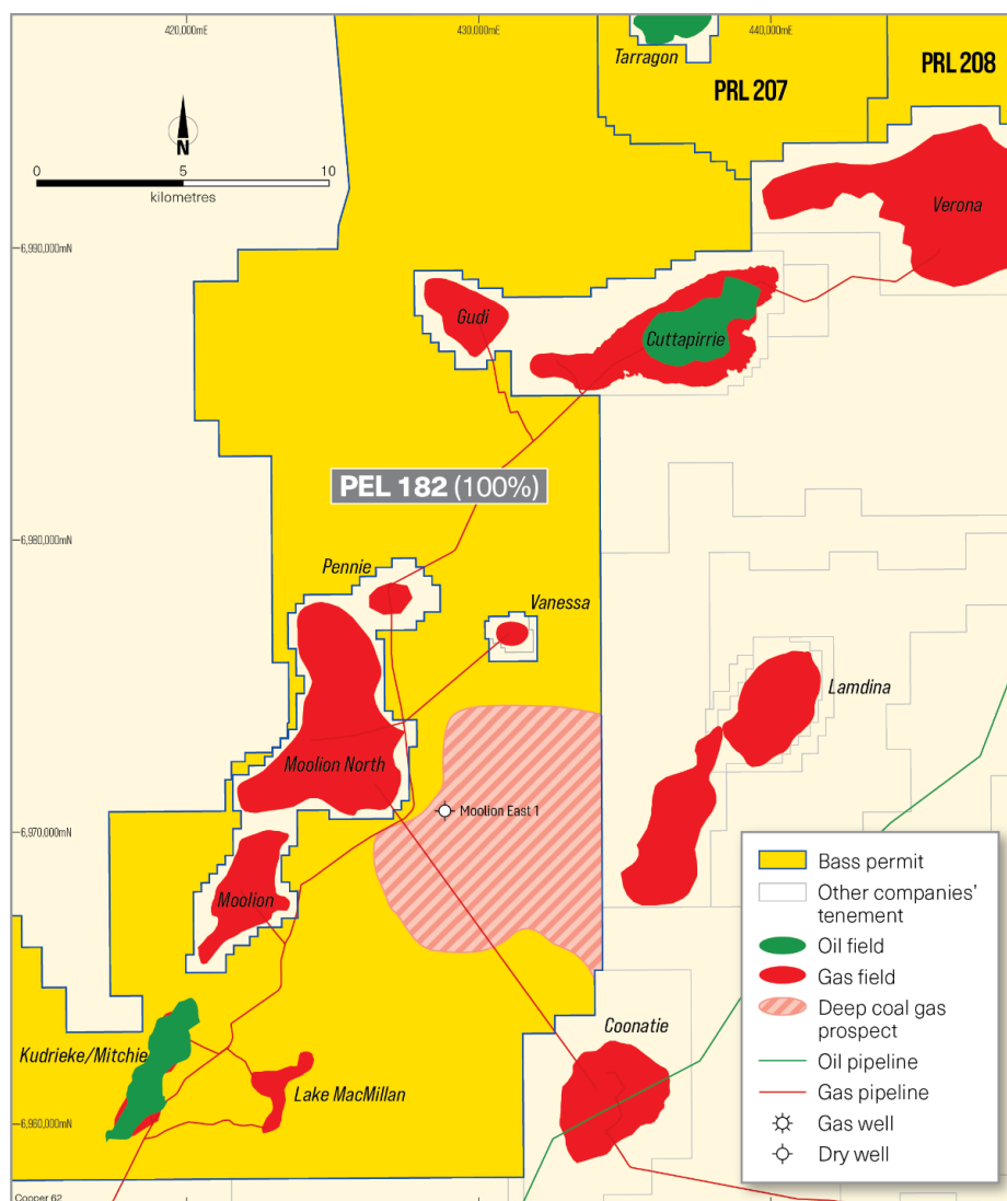
Figure 5: Map of Bass permit PEL 182 with drilled and producing nearby gas fields and pipelines
