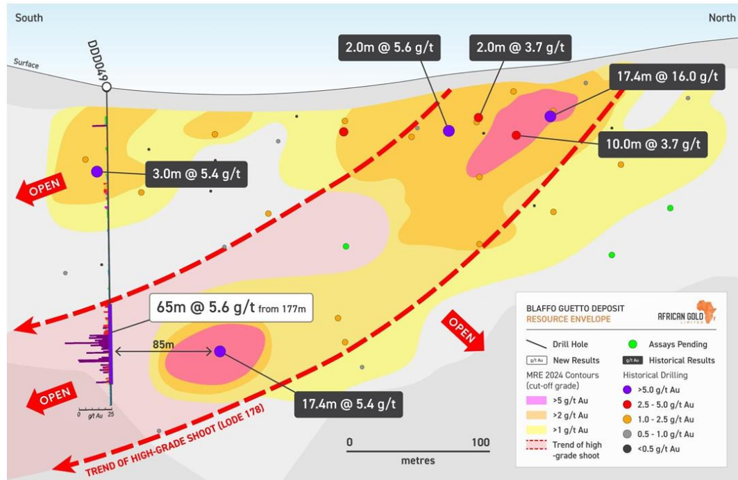
Figure 3: Long section of lode 178 showing the location of drillhole DDD049, the contours of the Mineral Resource (MRE 2024 data, ASX release dated 30 July 2024) and the interpreted south-westerly plunging high-grade shoot.
