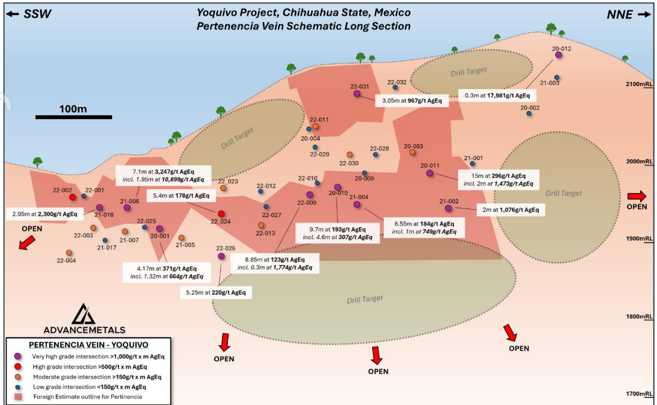
Figure 3. Schematic long section showing previous drill intersections at Pertinencia, colour-coded by silver equivalent multiplied by down hole interval (g/t x m AgEq). Selected intersections are also highlighted on the long section, as is the current Foreign Estimate outline and four key areas to identified four follow-up drilling (ASX AVM 3 March 2025). Silver-equivalents have been calculated as per footnote 1.
