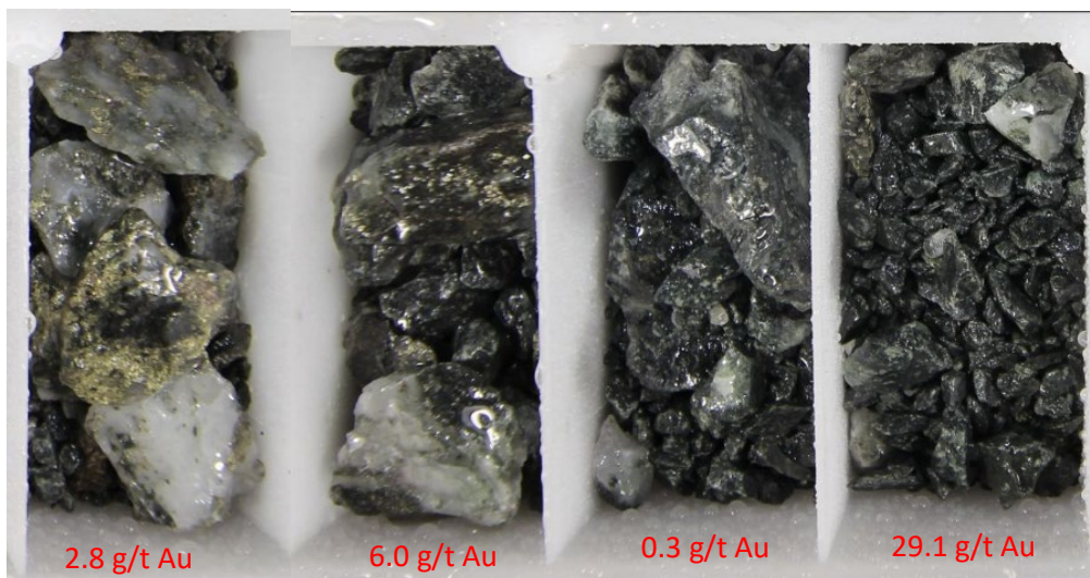
Figure 5: R24KP1234 reported 4m @ 9.6/t Au, 0.6% Cu, 9.5g/t Ag from 294m. Mineralisation associated with the high-grade lode is predominantly sulphides, 5%-20% Pyrite and 5-10% chalcopyrite, and quartz veining.
