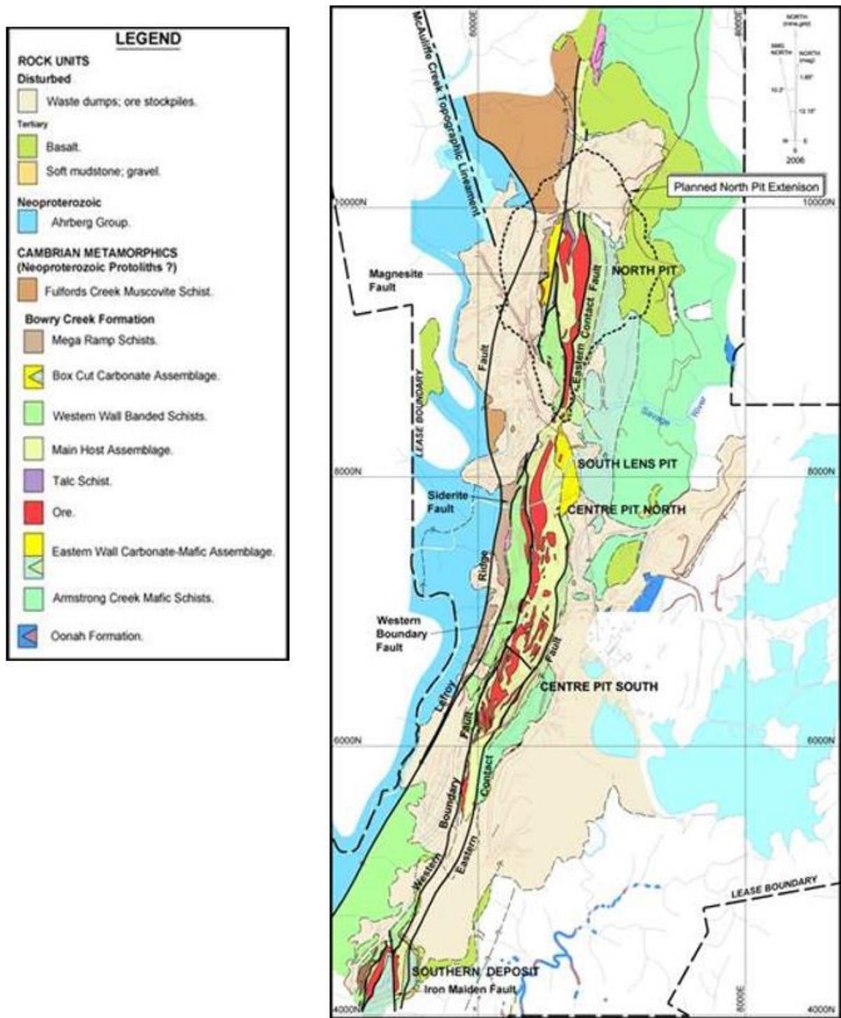
Figure 10 Regional Geology (2008)
