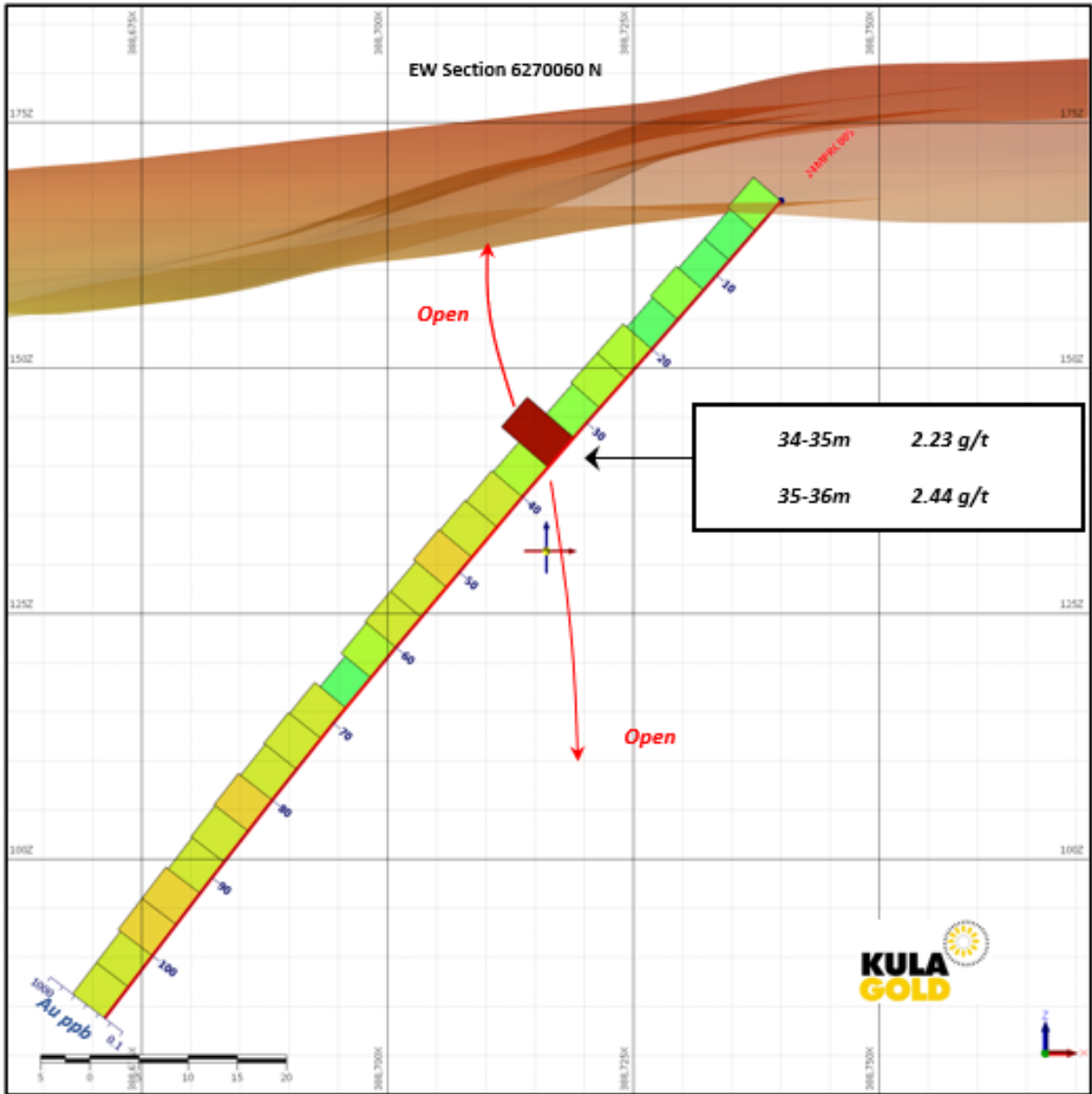
Figure 3: Mustang Prospect cross section with drillhole 24MPRC005.
