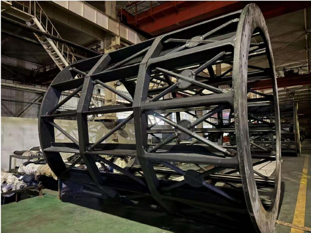
Picture 3: Feed and Discharge Assembly
