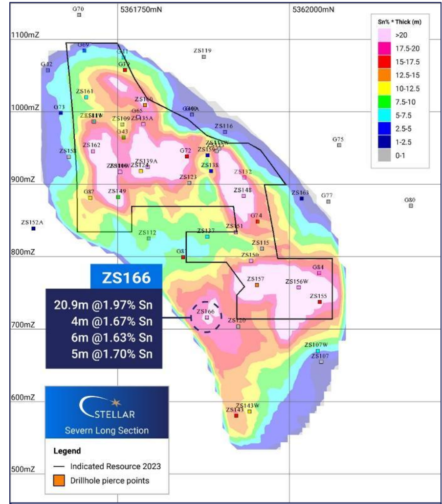
Severn Long Section looking west showing Sept 2023 Severn Mineral Resource as projected total of the multiple mineralised resource zones and drillhole pierce points coloured by Sn% * Thickness (historic holes & SRZ holes shown). GDA Z55
