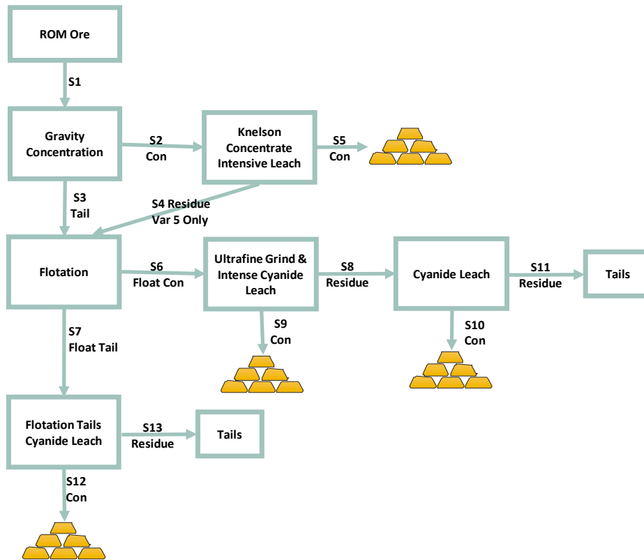
Figure 2: Test Work Process Flowchart
