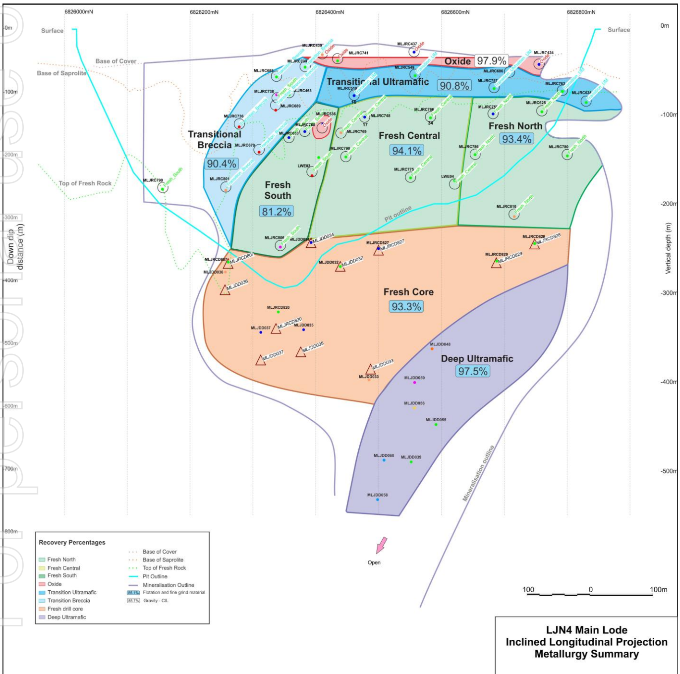
Figure 1: LJN4 eight metallurgical samples mineralisation types
