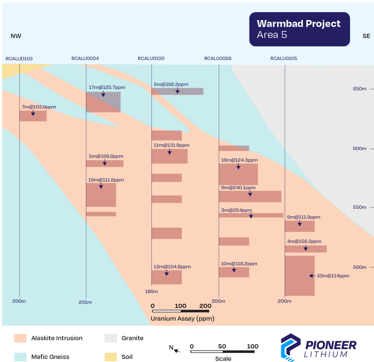
Figure 3: Cross section of the northeastern most drill line at area 5 showing significant uranium intercepts within the Alaskite body
