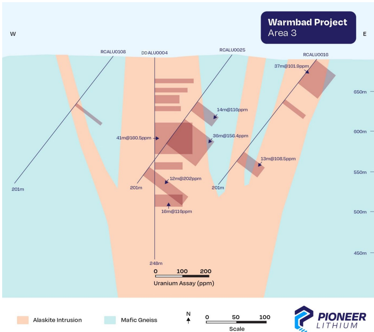
Figure 5: Cross section across the north of area 3 showing significant uranium intercepts within the Alaskite body
