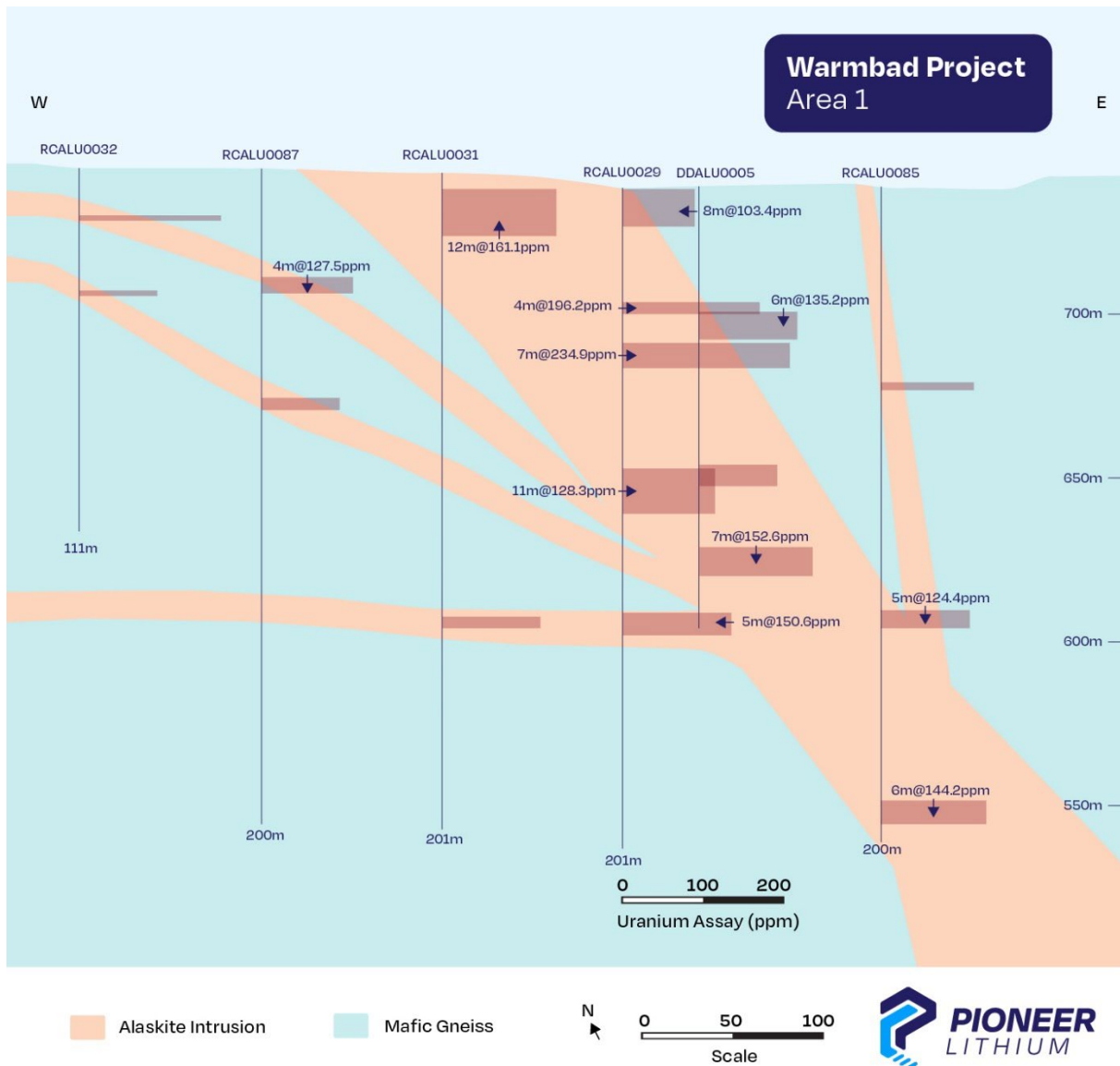
Figure 7: Cross section across the north of area 1 showing significant intercepts within the Alaskite body showing mineralisation open to the east and at depth.
