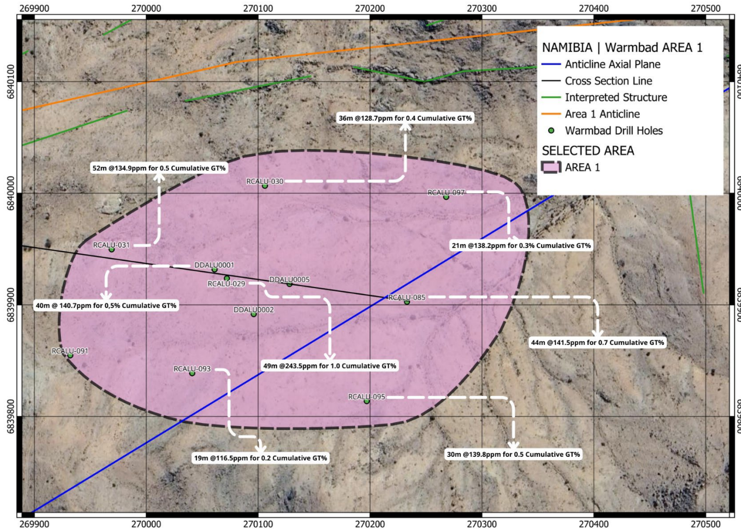
Figure 6: Area 1 zone of uranium mineralisation defined by historic exploration between 2007 and 2009. Diagram shows total uranium mineralisation intercepted in each drillhole and expressed as cumulative GT
