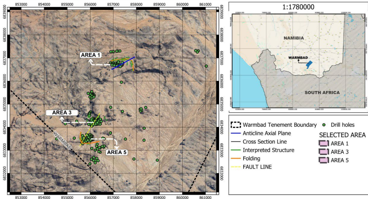
Figure 1: Overview map of the Warmbad Prospect showing historic drill hole locations and three areas of identified significant uranium mineralisation.
