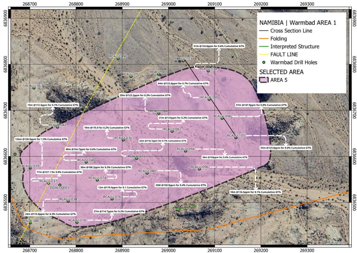
Figure 2: Area 5 zone of uranium mineralisation defined by historic exploration between 2007 and 2009. Diagram shows total uranium mineralisation intercepted in each drillhole and expressed as cumulative GT
