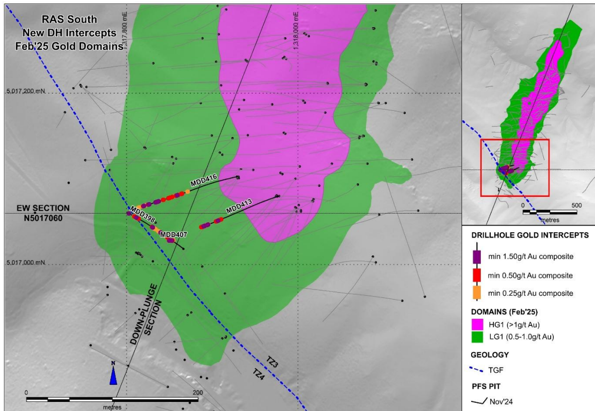
Figure 1. Plan of RAS South New Drill Intercepts vs Current Gold Domains.
