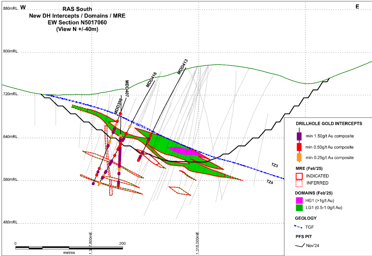
Figure 2. RAS South East-West Cross-Section N5017060
