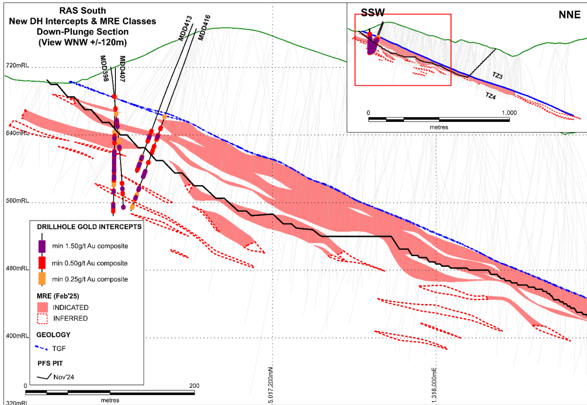
Figure 4. RAS South Down-Plunge Section Drill Intercepts vs MRE & PFS Pit
