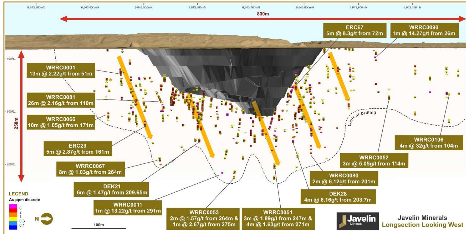
Figure 2 - Long Section showing significant gold intersection along with the main mineralised projected gold lodes looking west of the Eureka Pit
