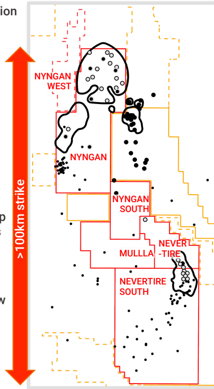
Figure 1: The Macquarie Arc is a proven Tier 1 terrane and Australia's foremost copper porphyry belt hosting a number of world-class mines The Northern Junee-Narromine Belt (NJNB) is a largely untested extension of the Macquarie Arc situated under the post-mineral cover
