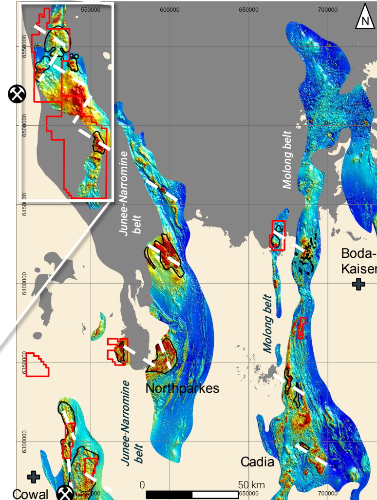
Figure 1: The Macquarie Arc is a proven Tier 1 terrane and Australia's foremost copper porphyry belt hosting a number of world-class mines The Northern Junee-Narromine Belt (NJNB) is a largely untested extension of the Macquarie Arc situated under the post-mineral cover
