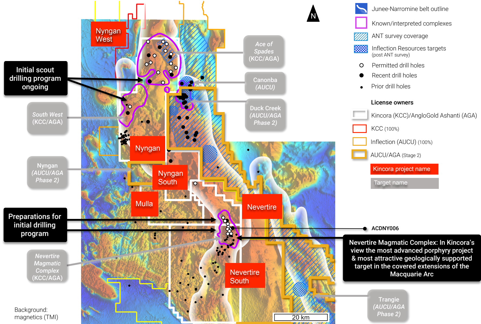
Figure 2: First phase drilling activities at Kincora’s Nyngan project are ongoing with activities initiated for initial drilling at the highly prospective Nevertire and Nevertire South projects
