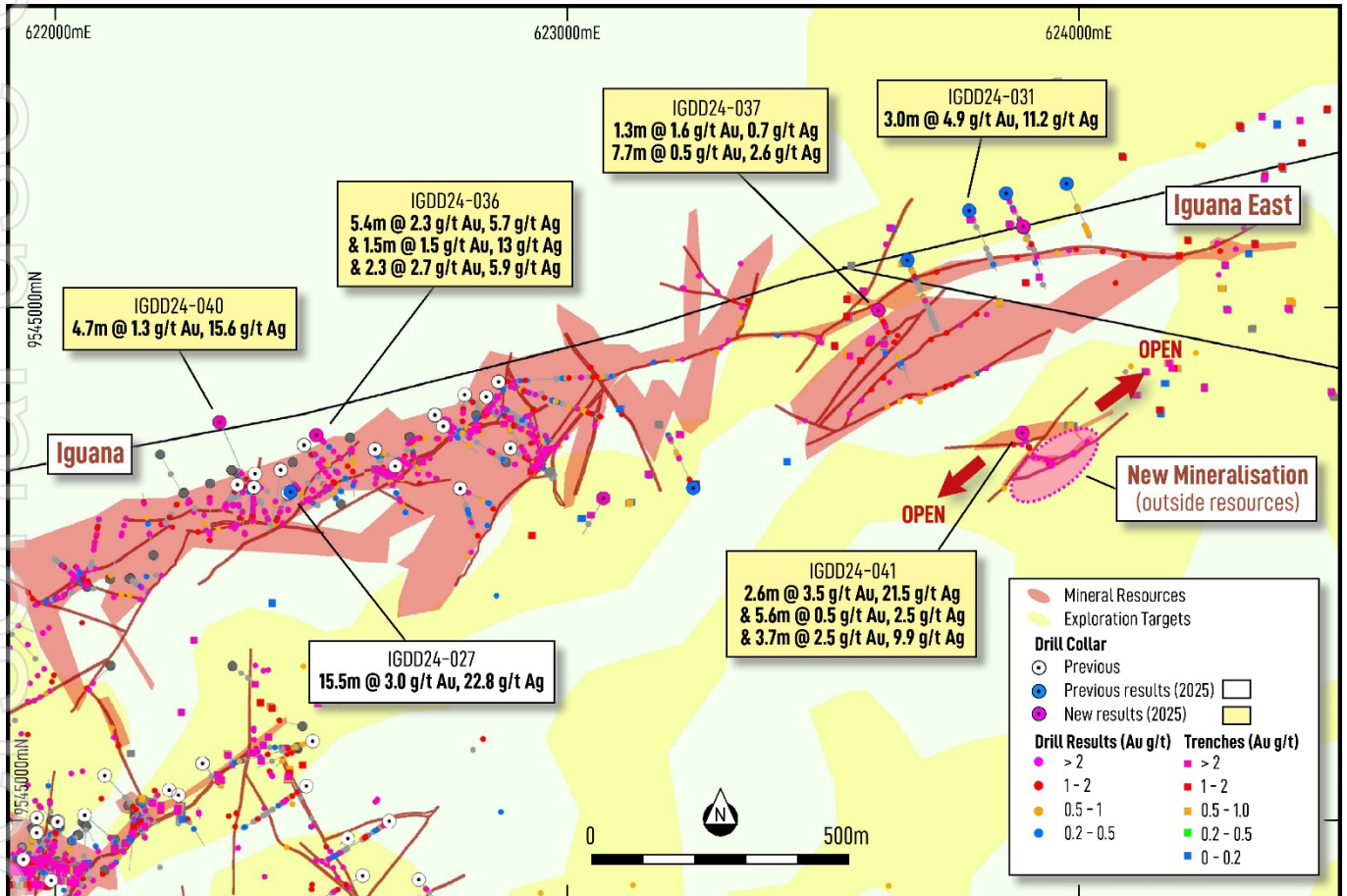
Figure 1. Iguana prospect displaying interpreted geology, modelled veins, resources, resource extensional targets, trenching and drilling completed and latest significant drill intercepts.
