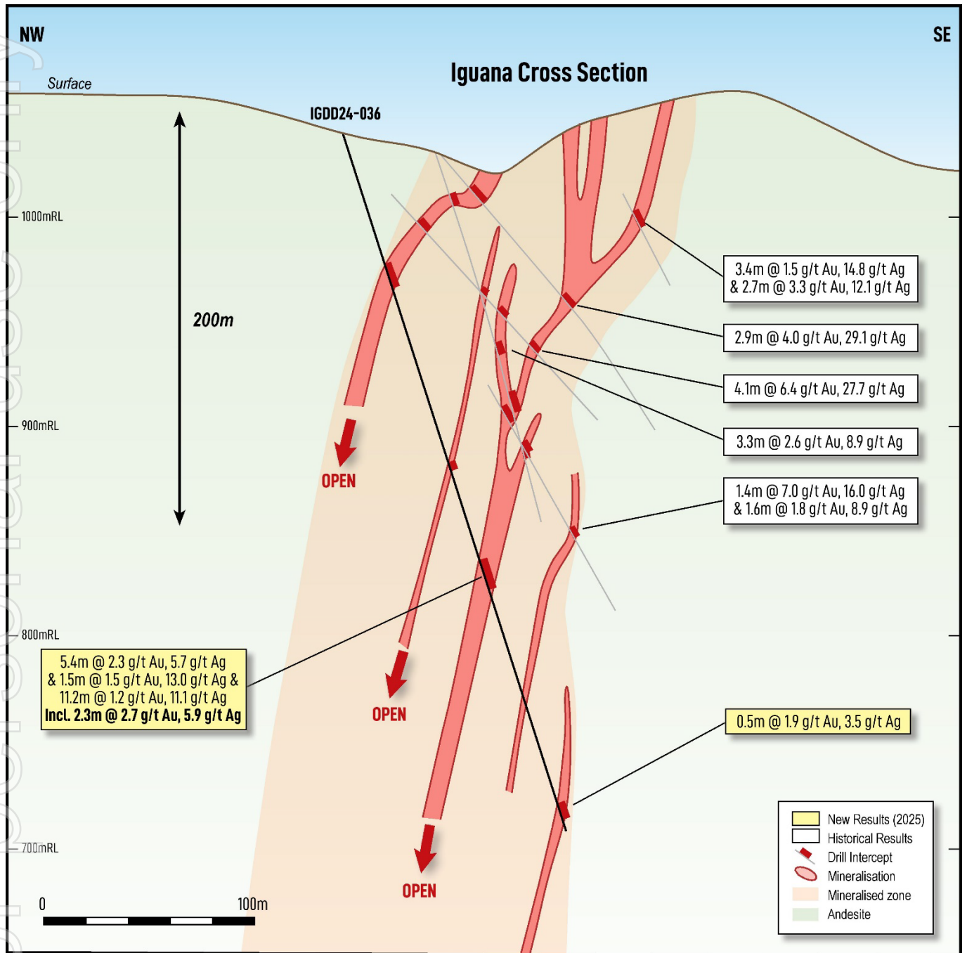
Figure 2. Iguana Cross Section looking northeast, showing geological interpretation, historical and new significant drill intersections. Note new drillhole IGDD24-036 assays returned, extending mineralisation down dip.
