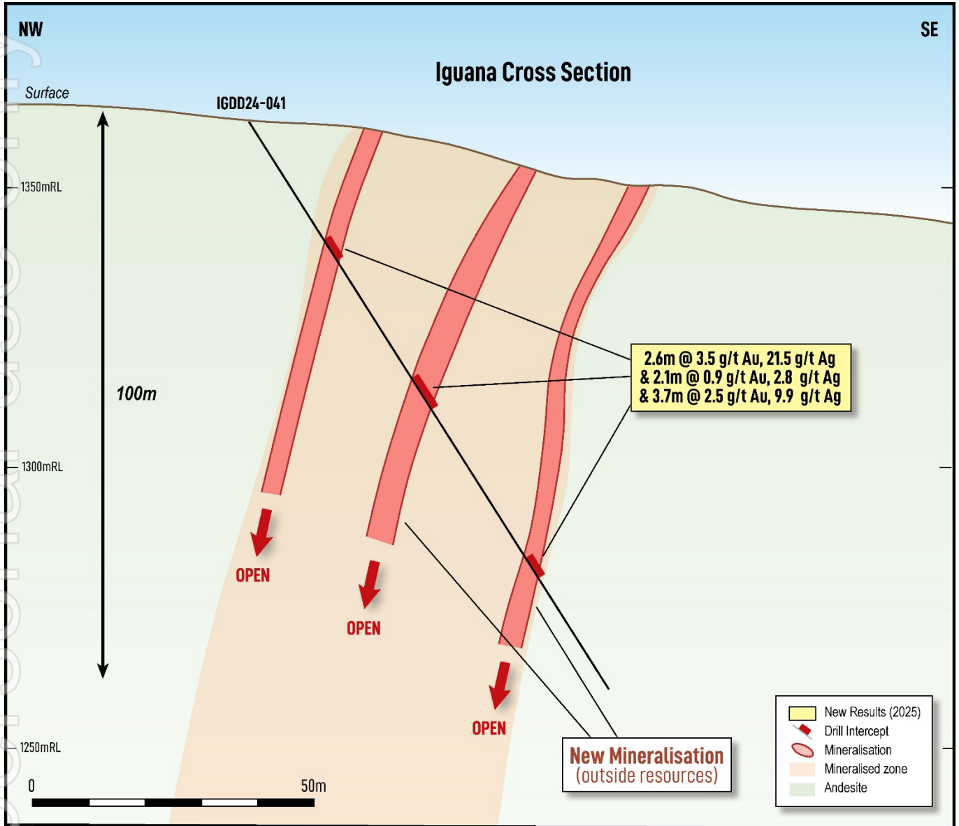
Figure 3. Iguana Cross Section looking northeast, showing geological interpretation, new significant drill intersections. Note new drillhole IGDD24-041 results, confirming and extending mineralisation from surface trenching and identifying two new mineralised veins from shallow depths outside current mineral resources.
