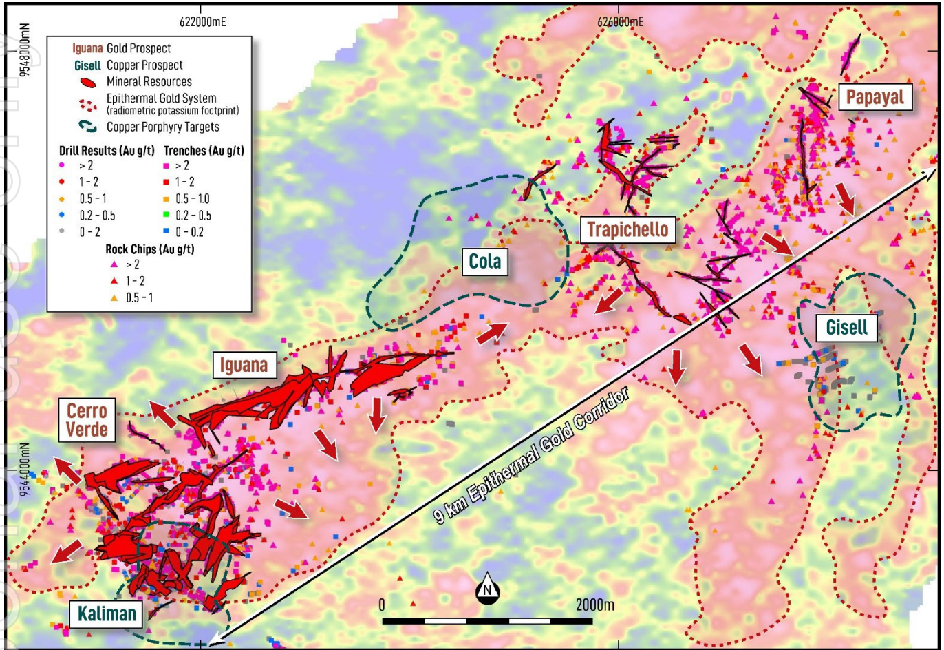
Figure 4. Dynasty Gold Project displaying Mineral Resources, epithermal gold system footprint as highlighted by radiometrics (potassium) and porphyry copper targets in relation to gold targets.
