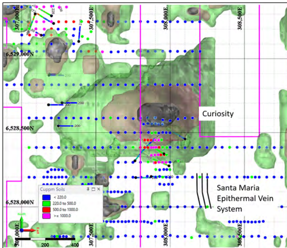
Figure 2. Curiosity Magneto-Telluric 3D Inversion Resistivity in plan view with north to top, MT Resistivity shells with green <math><100\Omega m</math>, pink <math><50\Omega m</math> and grey <math><35\Omega m</math> and soil geochemistry overlaid.
