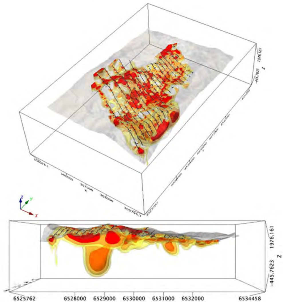
Figure 3. Llahuin audio-frequency MT survey. 3D inversion model resistivity isosurfaces (shells) at 100, 200 and 300 \Omega m (red, orange and yellow respectively). Looking from above toward NW and side on from the east (south to left hand side). The objective of the survey was to characterize the distribution of the resistivity parameter to a depth of around 1.4km, to image resistivity contrasts that might be associated with buried alteration or sulphide mineralization and/or other features of geological interest.
