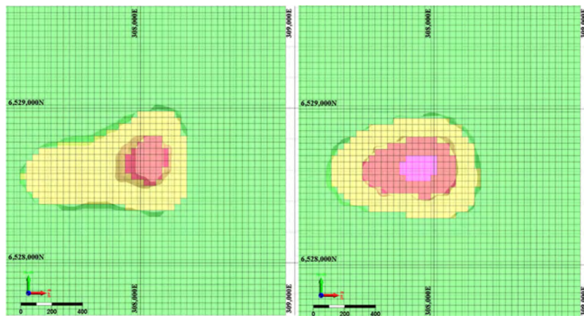
Figure 5. 700mRL and on the right-500mRL depth slices Llahuin Curiosity MT Resistivity- Green >100 \Omega m Yellow 50 \Omega m to 100 \Omega m red less than 50 \Omega m and pink <35 \Omega m
