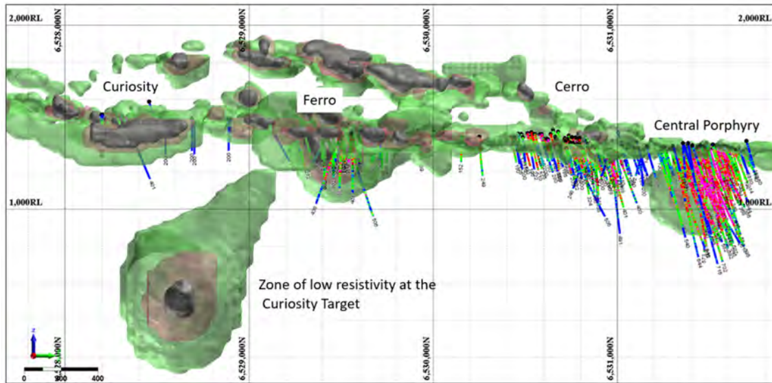
Figure 1 Llahuin Magneto-Telluric 3D Inversion Resistivity long section with north to right and MT Resistivity shells with green <math><100\Omega m</math>, pink <math><50\Omega m</math> and grey <math><35\Omega m</math>. Drill traces overlain.
