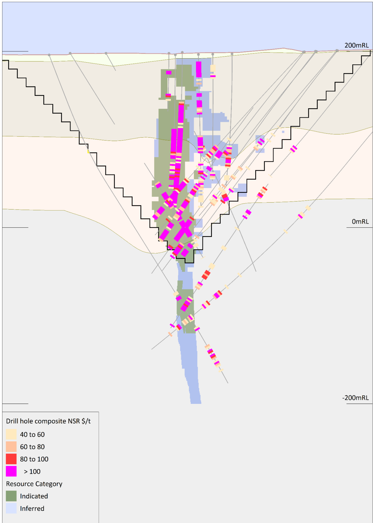
Figure 2 - Wagga Tank cross-section looking northeast
