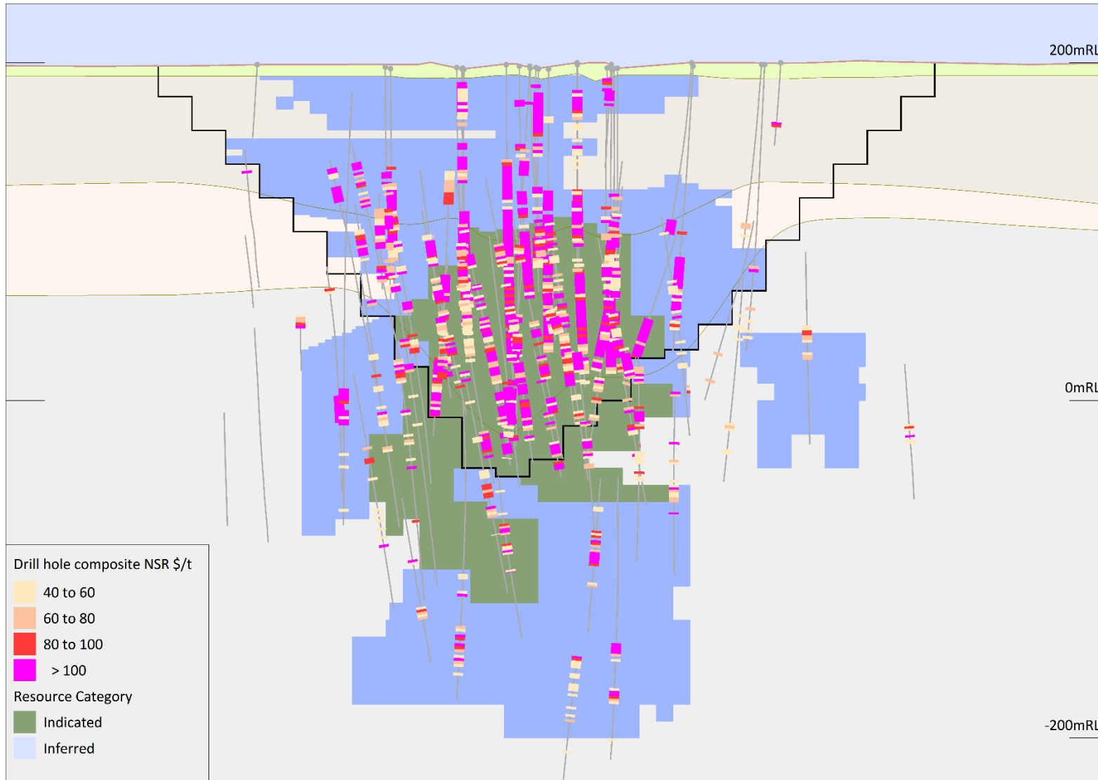
Figure 1 - Wagga Tank long-section looking northwest
