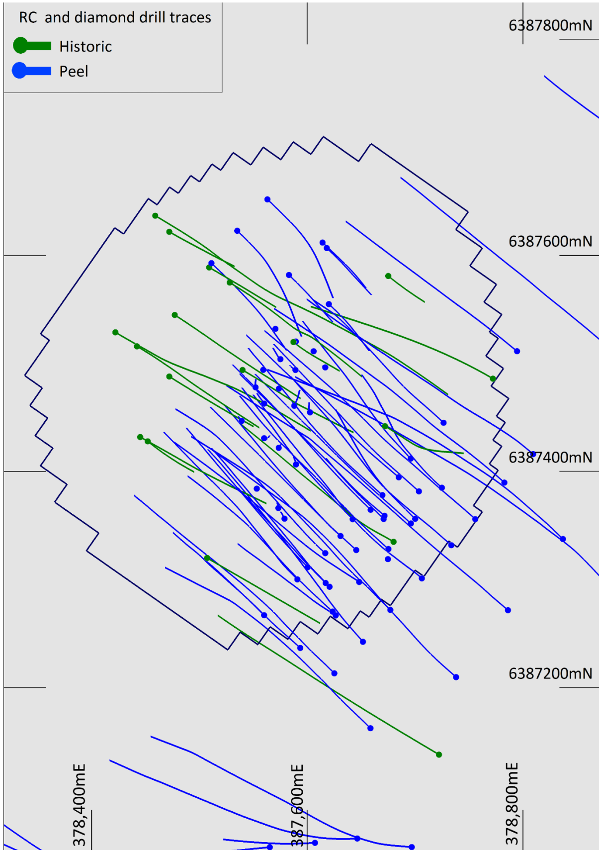
Figure 3 - Wagga Tank plan view
