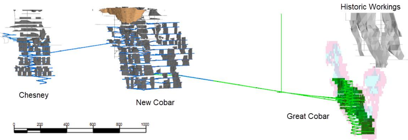
Figure 2: Mine layout – Full Design - Longsection
