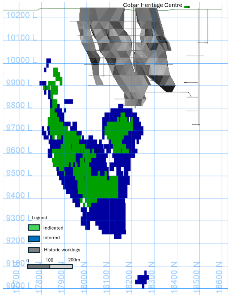
Figure 2 Long section of the Great Cobar Mineral Resource Estimate
