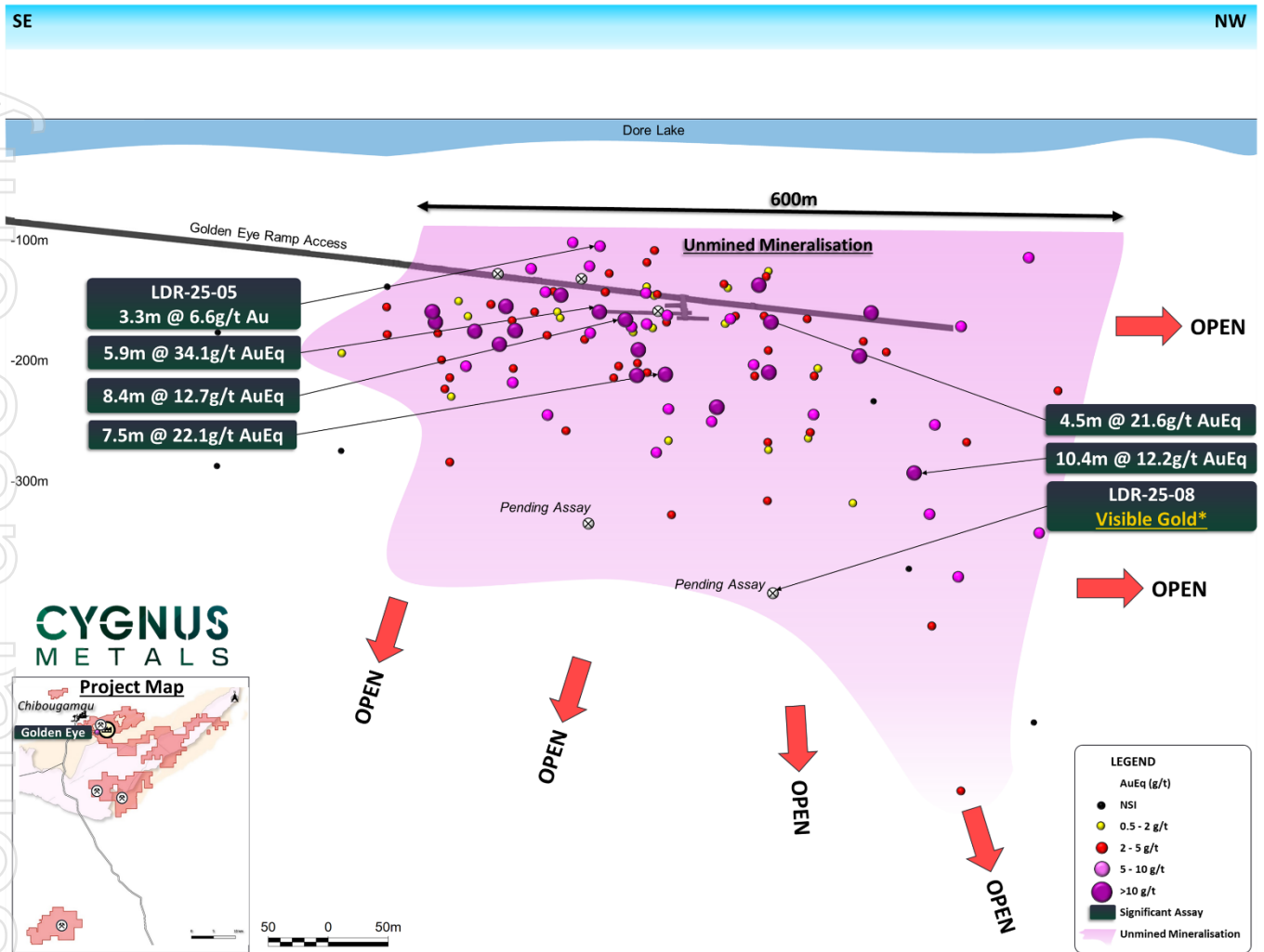
Figure 1: Long Section of Golden Eye over 600m of strike with significant high grade gold up to 34.1gt AuEq over 5.9m. Mineralisation is still open at depth, with visible gold intersected in LDR-25-08. Refer to Appendix A of this release for newly released drill intercept and ASX releases dated 15 October 2024 and 25 March 2025 for previously announced drilling results.
