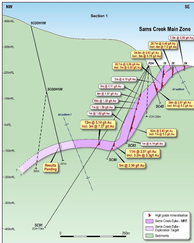
Figure 2: Schematic Cross-section 1 through the Main Zone mineralisation, showing SCDDH108 intersection.
