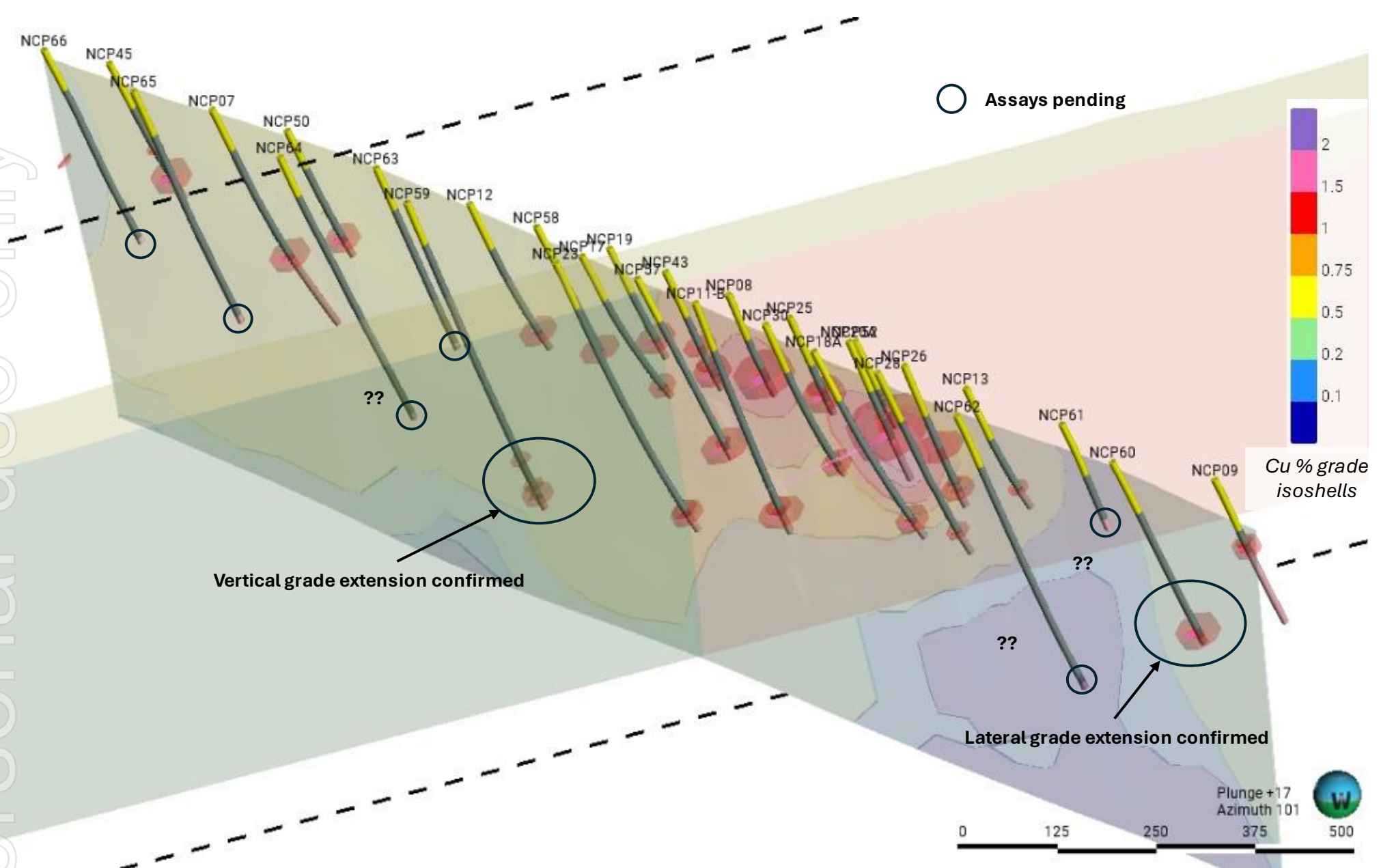
Figure 4. 3D extended cross section illustrating previous modelling grade shells with recent drilling and outstanding assay results highlighted.
