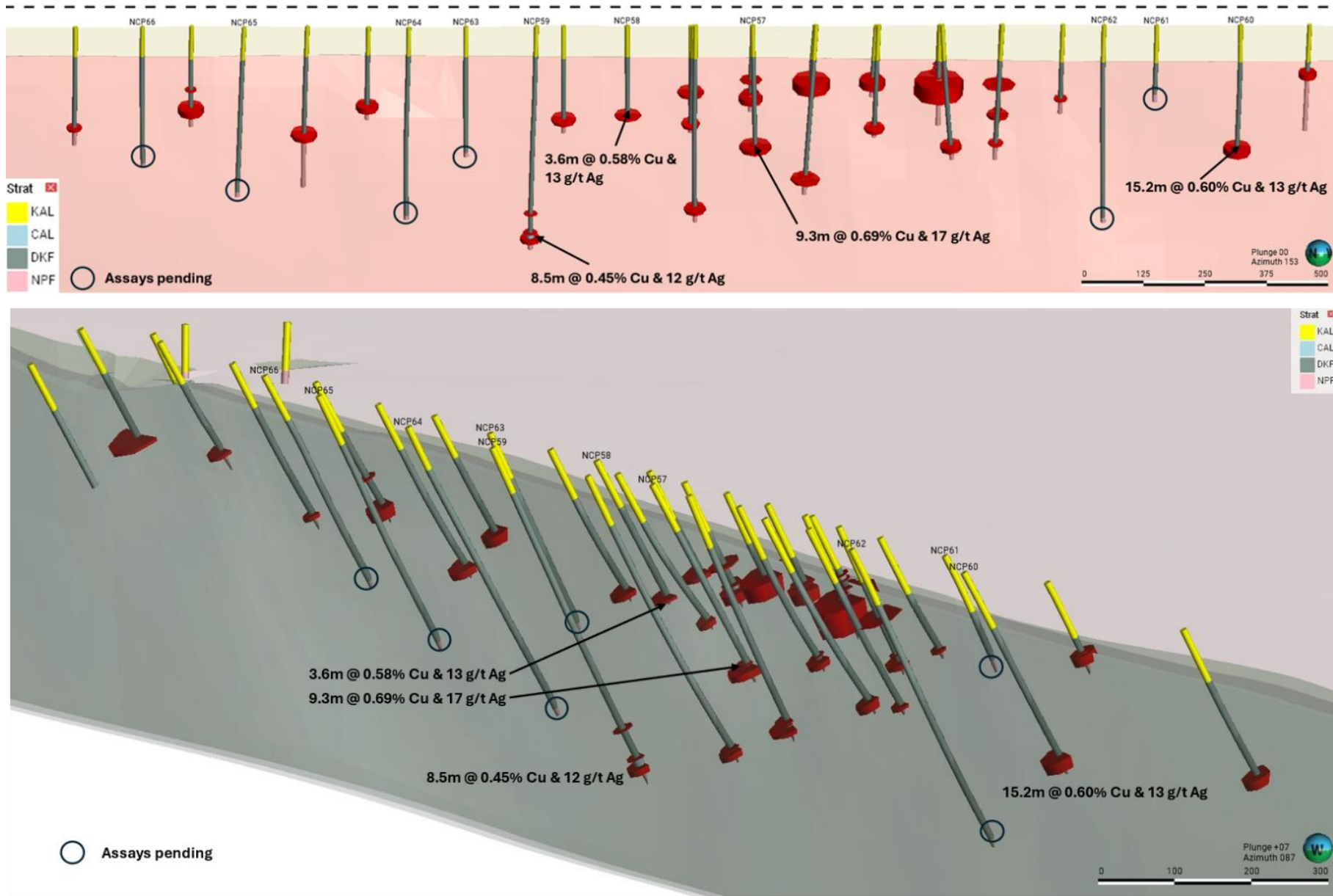
Figure 3. Long-section (top) and oblique view (bottom) illustrating recent and outstanding drill results.
