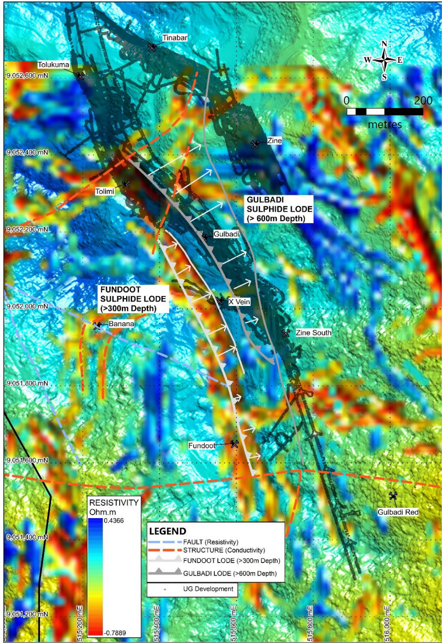
Presumed High Sulphide Conductivity Lodes (Blue) beneath the Tolukuma Mine
