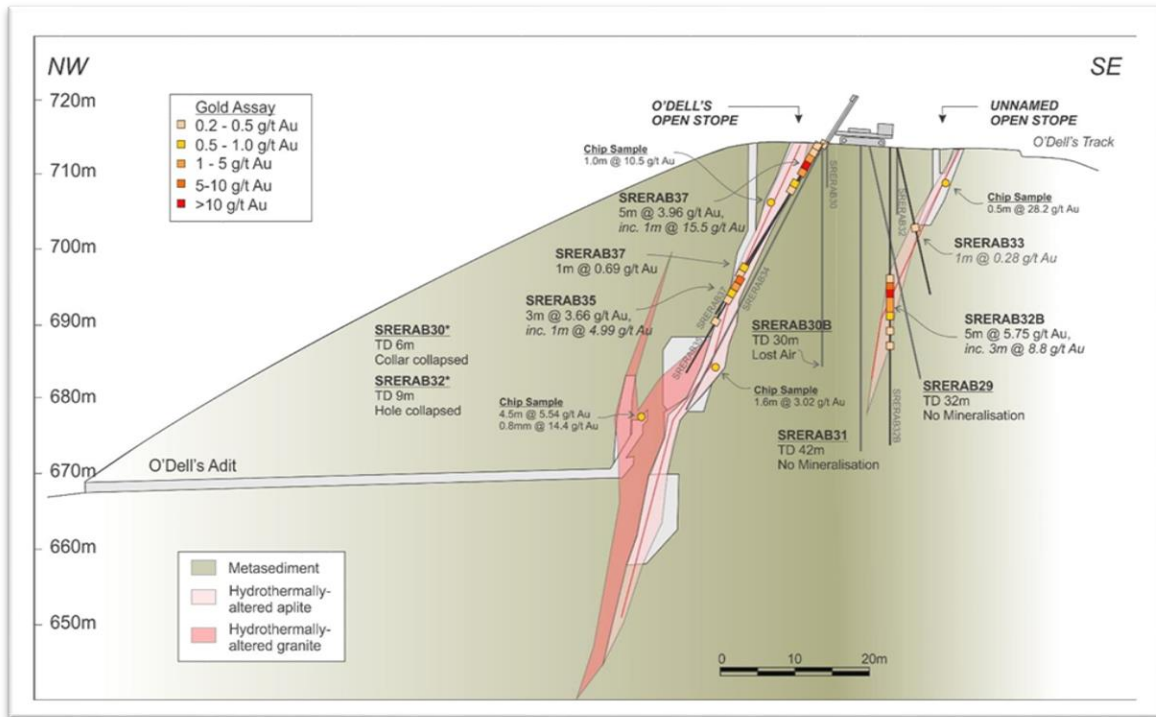
Figure 4: : Cross Section of drilling at Sandy Creek (O'Dells shaft) taken from Dart Mining ASX release 16th February 2021.
