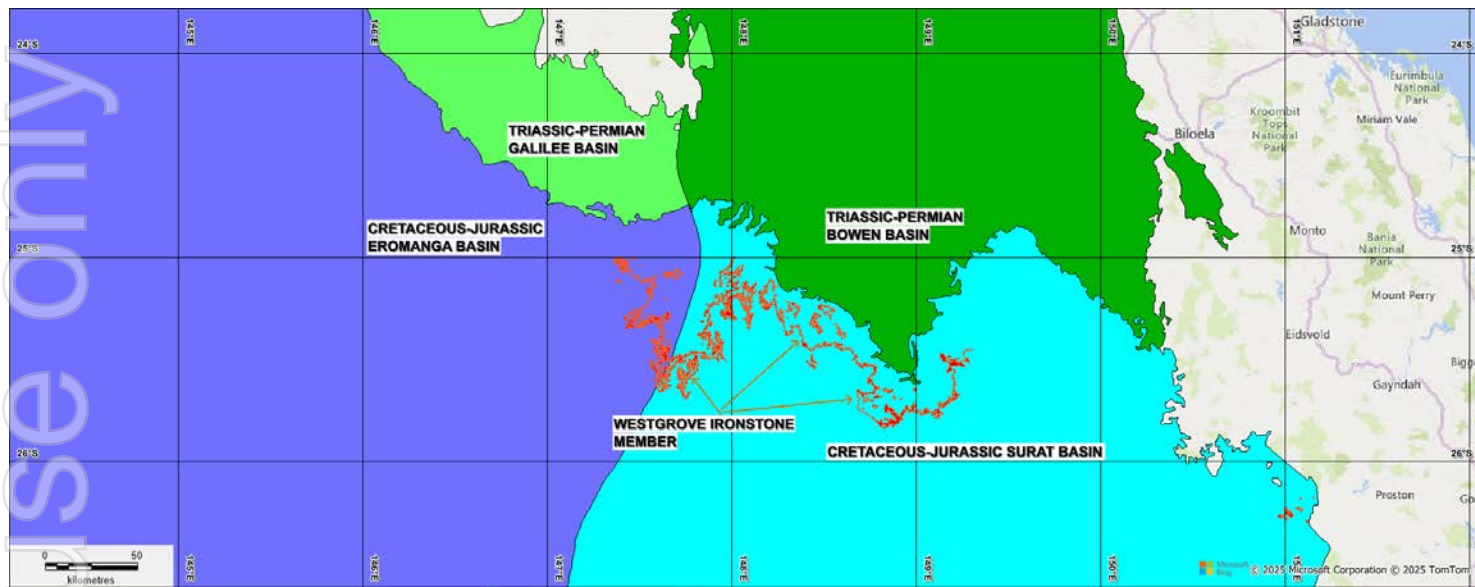
Figure 14 Location of the Westgrove Ironstone Member across the northern margin of the Surat and Eromanga Sedimentary Basins
