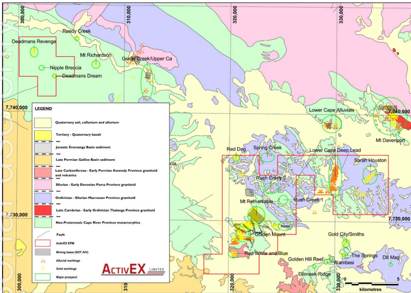
Figure 16. ActivEX Limited Pentland Gold Project regional geology and key prospects.
