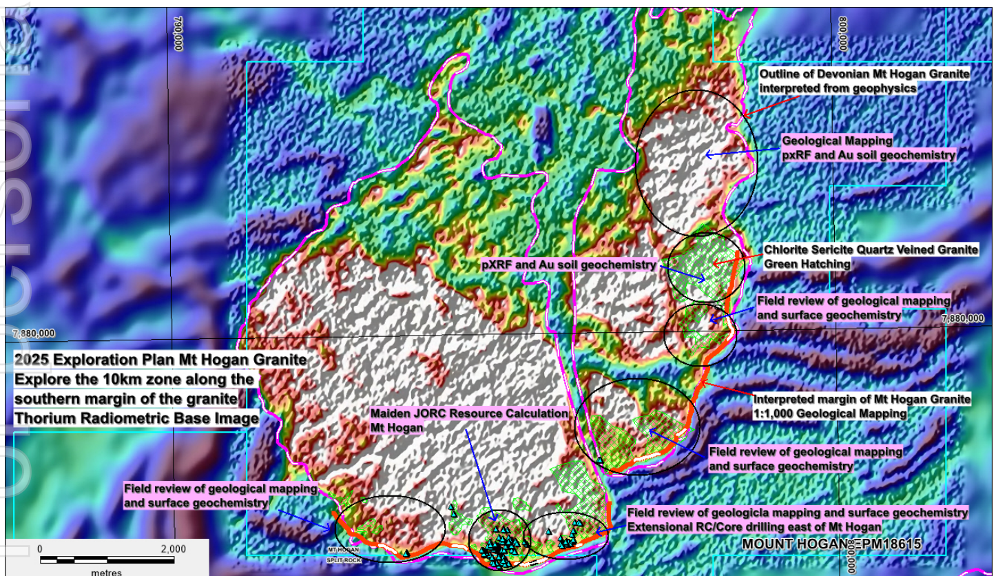
Figure 3 Thorium Radiometric Base Image detailing the 2025 Exploration Plan for Mt Hogan Granite, specifically focusing on the 10km zone along the southern margin of the granite.
