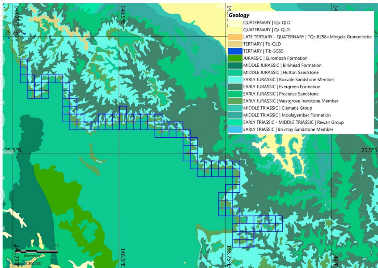
Figure 15. ActivEX Doonkuna Local Geological Setting – Note the tenement application is targeting the Westgrove Ironstone Member
