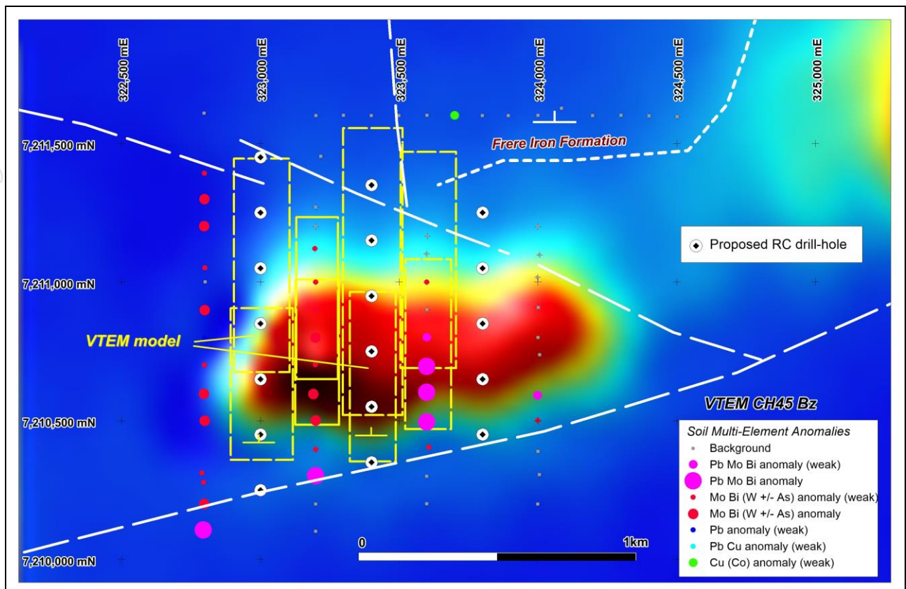
Figure 13: Mt Davis: Late Time VTEM Image showing soil anomalies and proposed RC drilling.
