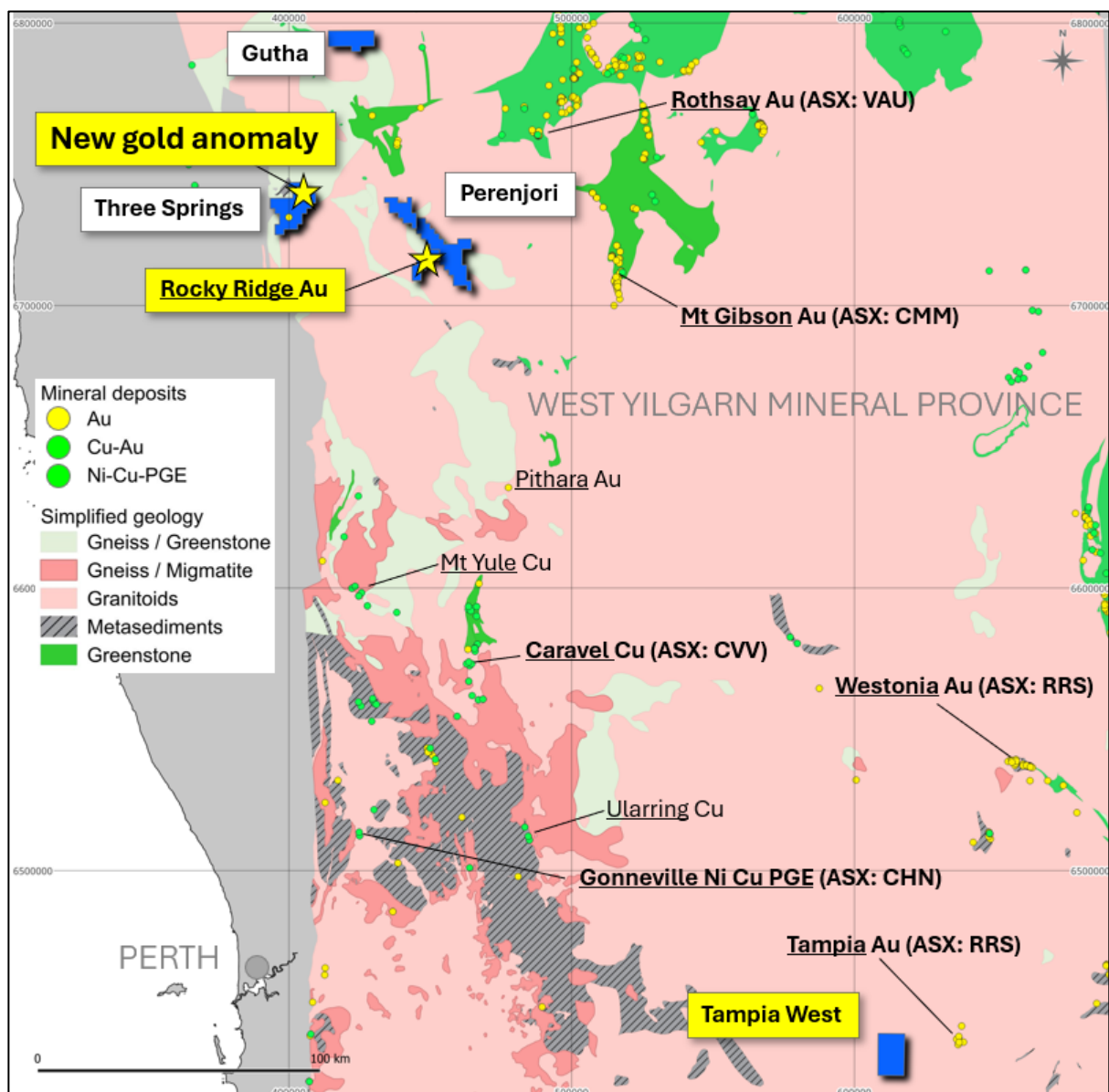
Figure 2. Simplified GSWA Interpreted bedrock geology showing Engex licences and recent mineral discoveries.
