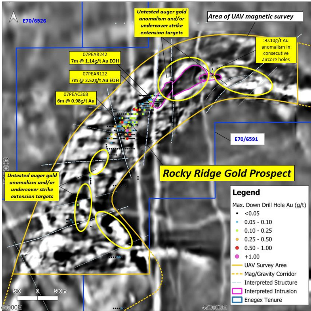
Figure 5. Rocky Ridge Prospect – Historical drill collar positions indicating maximum down hole gold values from >9m depth on Enegex’s UAV aeromagnetic imagery draped over public aeromagnetic imagery. Main target areas indicated in yellow and are often coincident with untested bedrock and areas below deeper cover.
