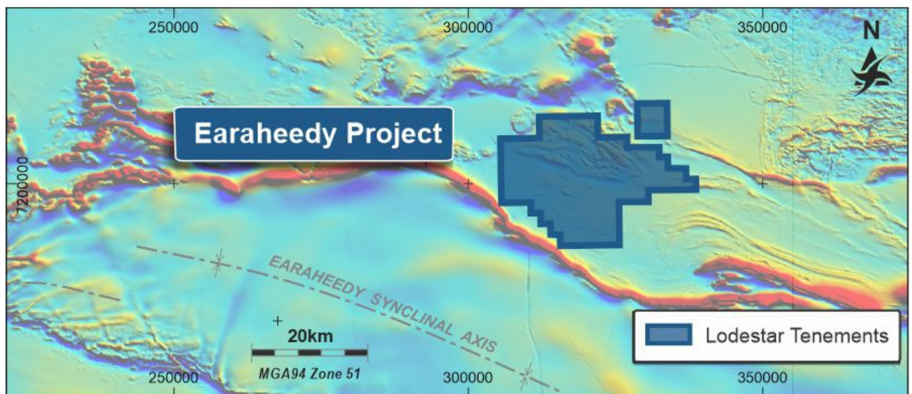
Figure 3: Earaheedy Project tenement areas on aeromagnetic background.
