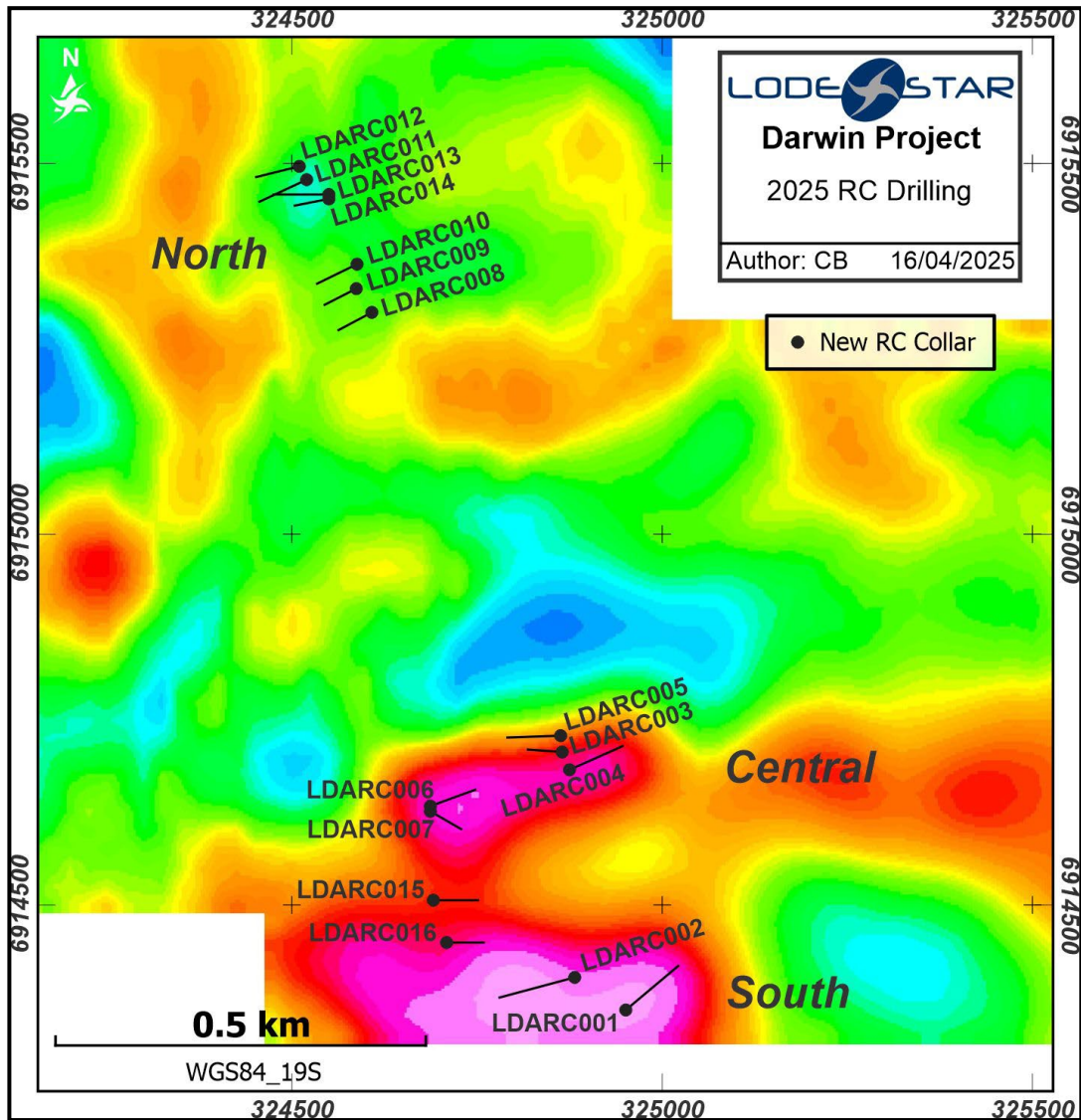
Figure 2: Completed drill hole traces projected to surface on aeromagnetic background (tmirtp 1vd)
